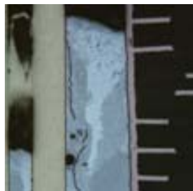
Insufficient vertical fill: microsection polarized light contrast.
