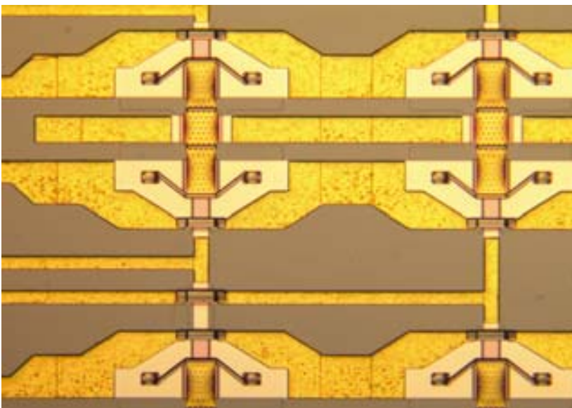
Figure 1: Photo and REM picture of a device acting as variable capacitor. The thin Ni membrane is free movable between the signal line below and the thick Ni electrodes above.
