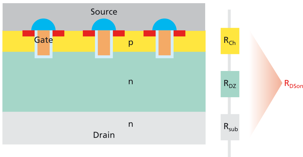
Figure 1: Schematic of a Trench-Gate PowerMOS device. The main contributing serial resistances R_{\text{Ch}} , R_{\text{Dz}} and R_{\text{Sub}} to the On-resistance R_{\text{Dson}} are shown.
