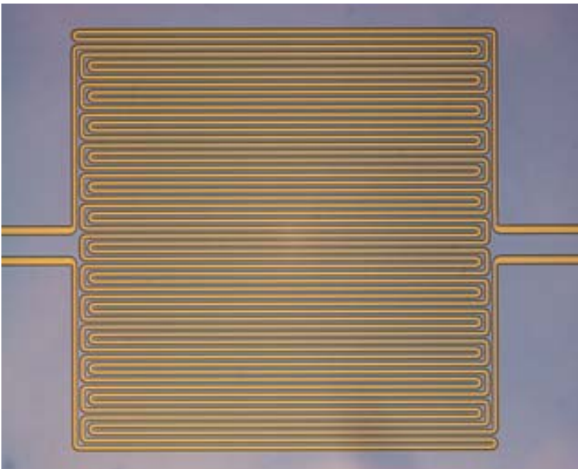
Figure 1: Meander structure of two resistance lines with 5 \mu\text{m} lines and spaces on a thin membrane.
