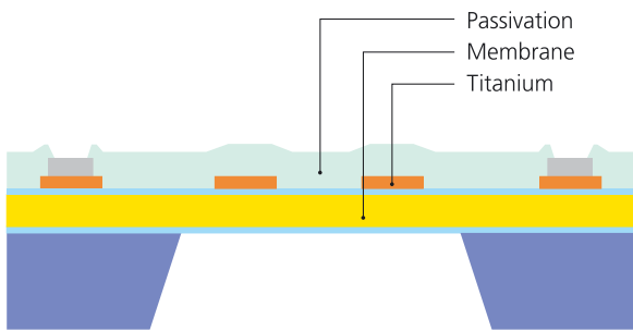
Figure 2: Cross-section of the membrane.
