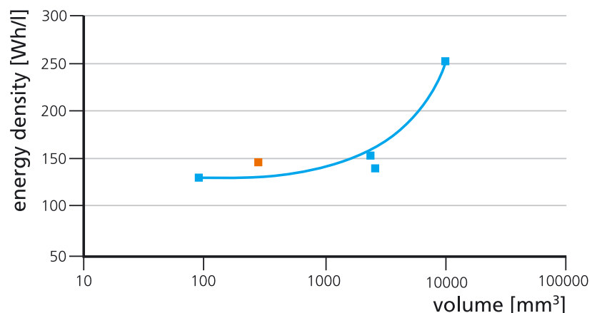
Figure 6: Energy density of commercial rechargeable batteries as a function of battery volume (orange: ISIT).
