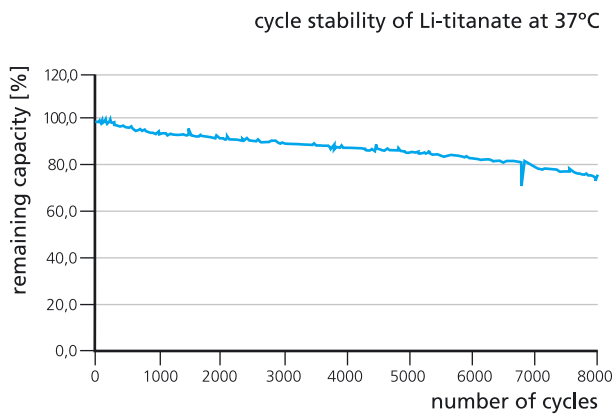
Figure 3: Cycle test of a Li-titanate cell (2,3 V, 37 °C).
