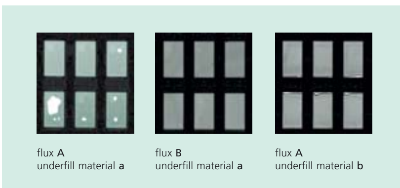
Figure 1: Investigation of voids with ultrasonic microscopy for different combinations of flux and underfill material.
