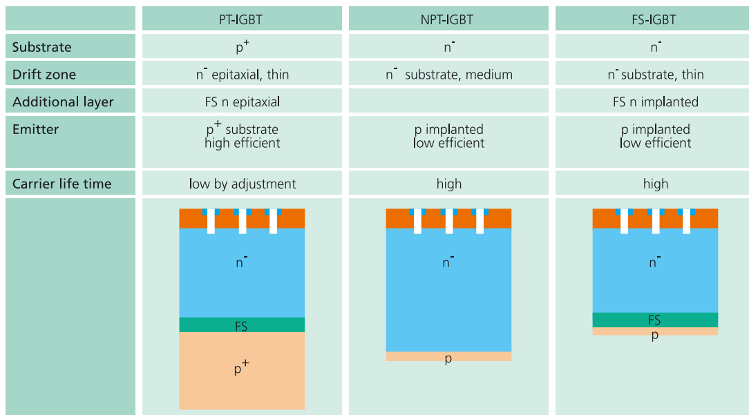
Figure 1: Overview on different Trench IGBT concepts.
