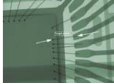
Figure 6: Real-time target alignment and measuring using x-ray and special set-up station.
