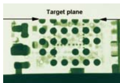
Figure 3: Radiographic image of hidden target, a row of solder balls on a CSP-component.
