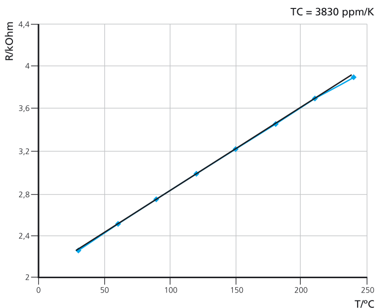
Figure 4: TC measurement of a Ti/TiN resistance.
