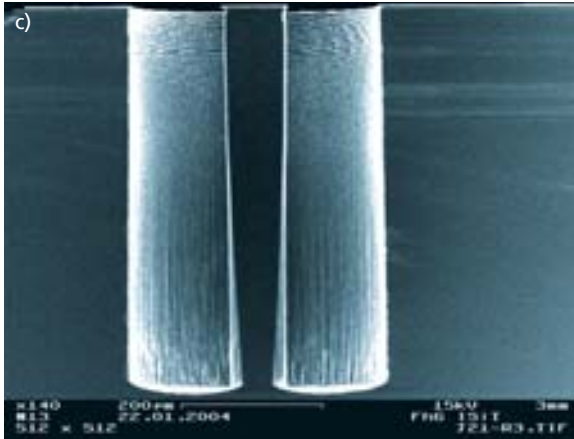
c) The donut structures are etched approx. 550 \mu\text{m} deep into the silicon wafer. Filling the donut structures was more difficult than using pin type wafers.
