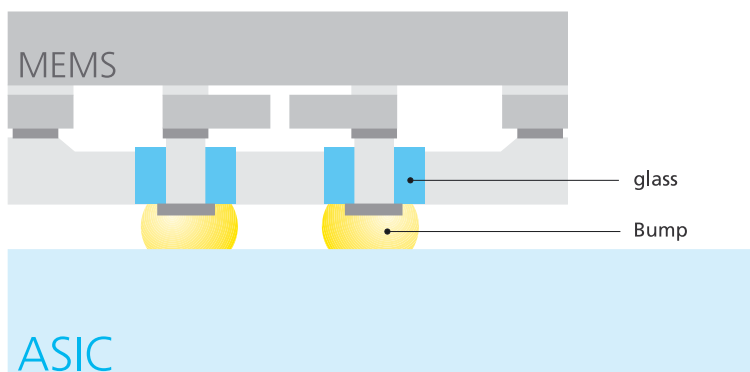
Figure 1: Electrical feedthroughs in the cap wafer enable the use of flip chip process for the connection of MEMS to the external electronic circuits.
