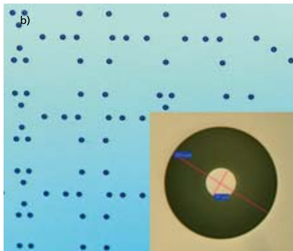
Figure 4: a) and b) Ring type silicon/ glass wafer – Small "donut"-shaped glass rings surround a silicon centre pin which forms the feedthrough contact.
