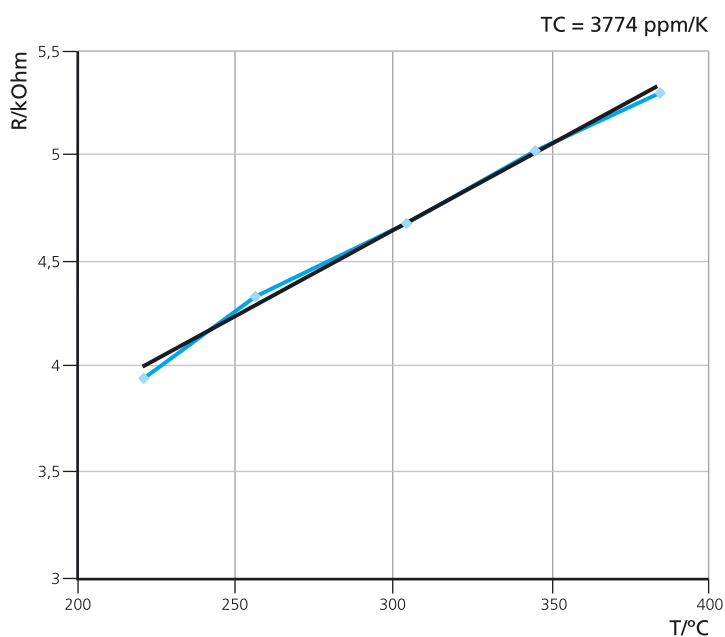
Figure 7: Measurement of the temperature coefficient TC by external heating of the chip.
