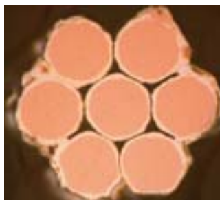
Figure 10: Status quo of the braided wire before dipping 1000x (micro section).
