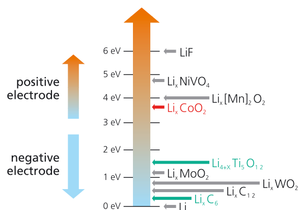
Figure 2: Electromotive series of lithium compounds (green arrows: anode materials, red arrow: cathode material).
