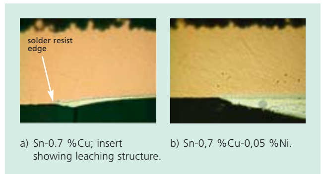
Figure 5: Effect of solder alloy on copper leaching; soldering at 255° C, low residue no-clean flux.
