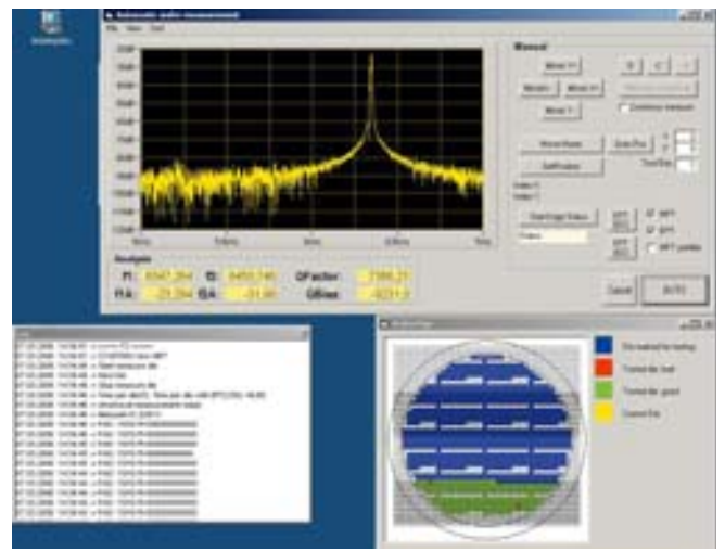
Figure 6: Graphical User Interface of the automatic wafer endtest.
