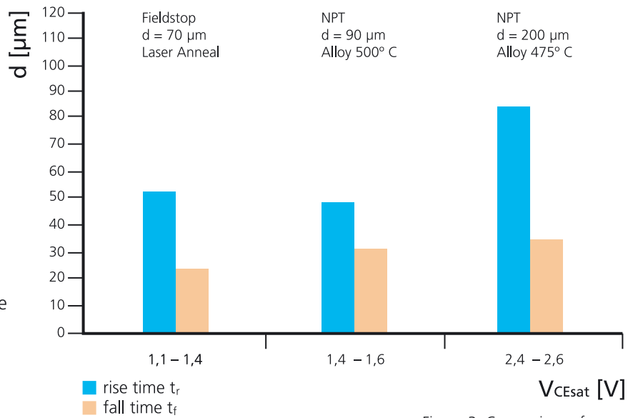
Figure 3: Comparison of electrical results for different Trench IGBTs.
