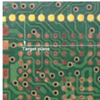
Figure 2: Printed Circuit Board with visible target, a row of microvias.
