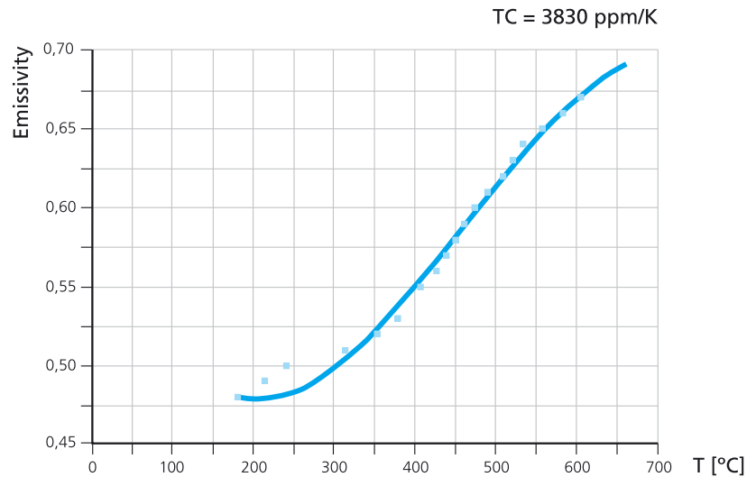
Figure 3: Emissivity as a function of temperature of a chip mounted on a heating block. The chip was completely processed except membrane etching to assure a good heatconductance.
