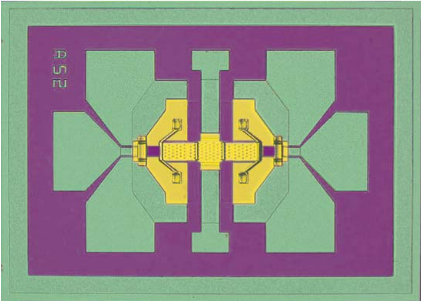
Figure 2: Photo of a capacitive RF-MEMS switch. The thin Ni membrane is supported by thick spring-type Ni anchoring structures compensating thermally induced stresses. To avoid high voltages on the signal line electrically isolated actuation electrodes are embedded in the ground area.
