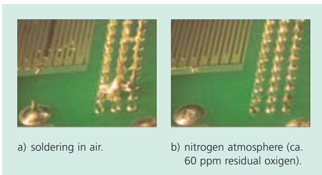
Figure 4: Effect of atmosphere on bridging; Sn-3.5 % Ag at 265° C, low residue alcoholic no-clean flux.
