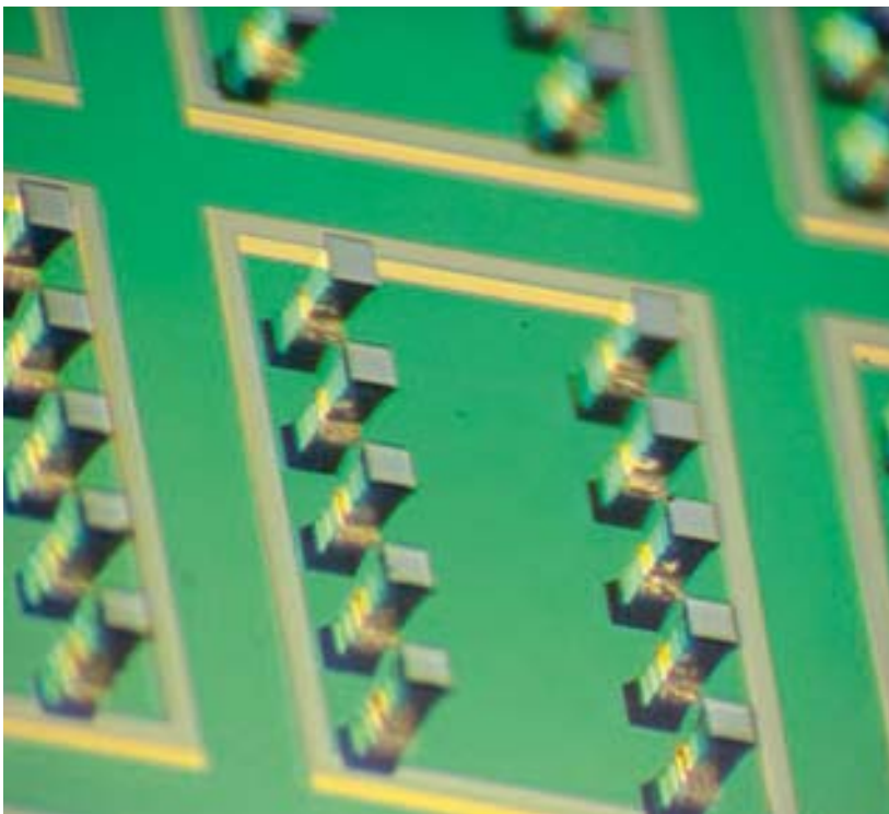
Figure 6: In this experiment, a feedthrough wafer was bonded on a wafer with gold pads. Both the silicon pins and the pads on the second silicon wafer were covered with 1 \mu\text{m} thick gold. Due to the reaction of the silicon in the pins, a gold/silicon alloy is formed during the bonding process and covers the pads.
