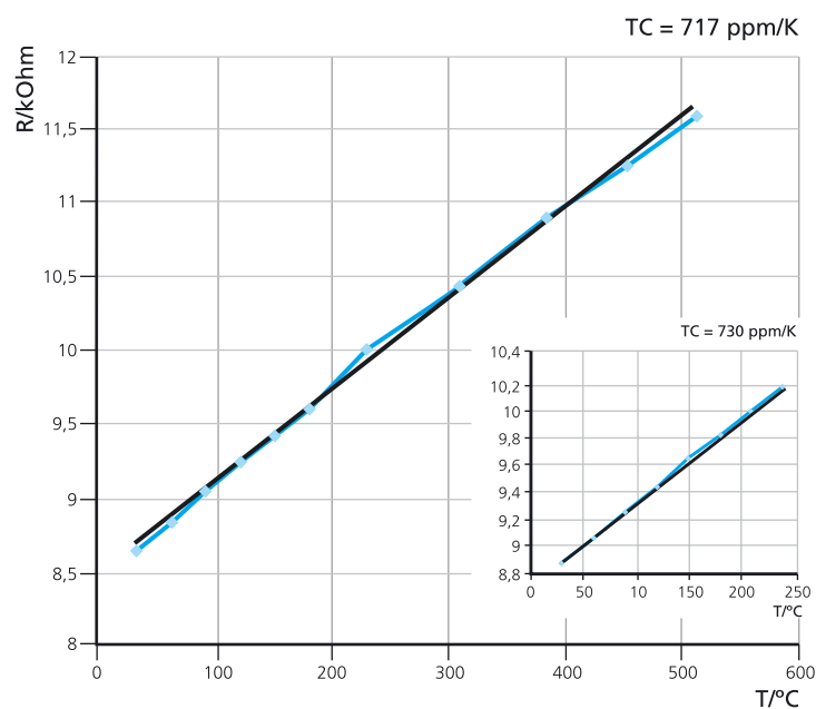
Figure 8: Calculation of the TC of TiN from the temperature dependence of the resistance for internal heating (30° C–180° C) and external heating (230° C–520° C). In the inset the calculation of the TC from internal heating (30° C–240° C) only is shown.
