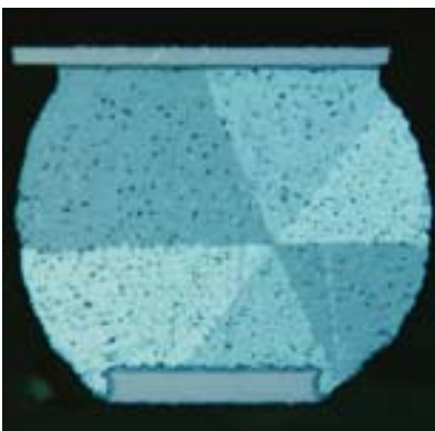
BGA ball: microsection polarized light contrast.
