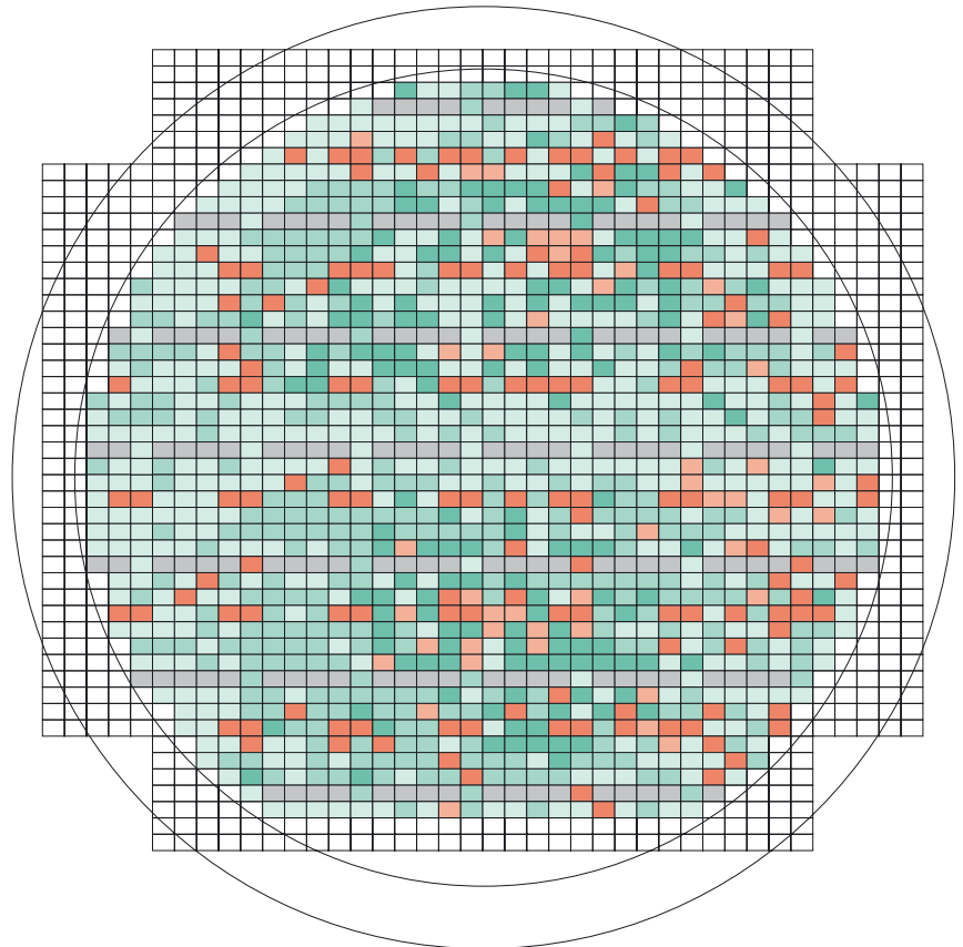
Figure 7: Wafermap of a tested MEMS wafer.
