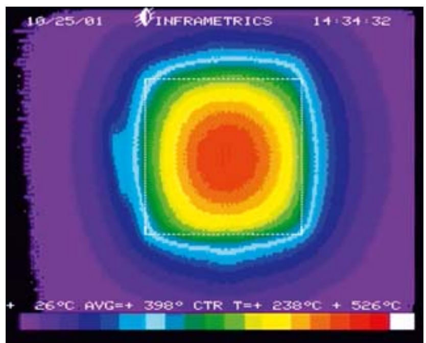
Figure 6: Infrared image of the membrane (area between the dashed lines), internally heated. The mean temperature of 398 °C is an integrated value over all areas with different temperatures.
