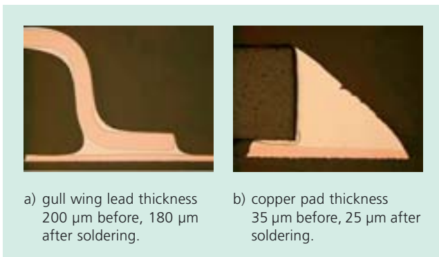
Figure 3: Copper leaching after double wave; Sn-3.5 % Ag at 265° C, low residue alcoholic no-clean flux.
