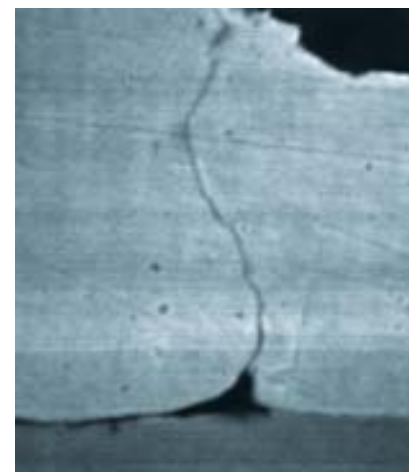
Figure 9: SEM image of wedge bond with crack.
