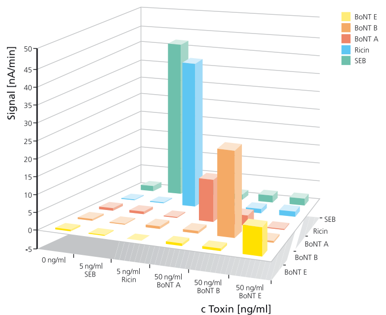
Figure 3: Signals of 6 measurements with one toxin per sample on the toxin array chip.
