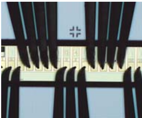
Figure 4: Needles of the probecard in contact with the sensor pads.
