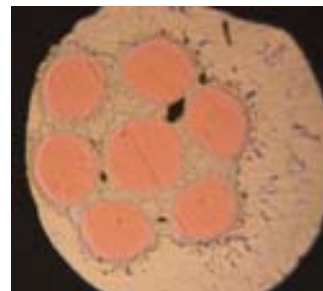
Figure 12: SnAgCu 1.3 – lower dissolution rate because of copper saturation in solder alloy 1000x.
