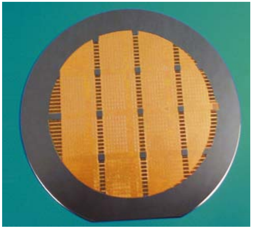
Figure 5: First bonding of a pin-type feedthrough wafer with a silicon wafer. The second wafer was covered with a gold layer (1 \mu\text{m} thick), while on the composite Si/glass wafer the silicon pins were also covered with gold.
