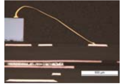
Figure 7: The entire length of the 20\mu\text{m} gold wire is visible in the cross section.
