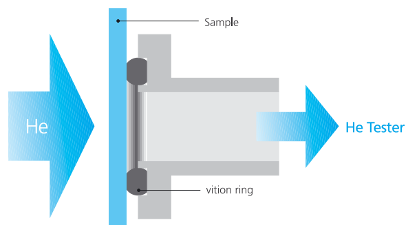
Figure 7: Scheme of the experimental set up to measure the leakage of different feedthrough samples.
