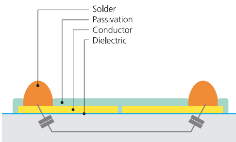
Figure 1: Cross sectional drawing of a chip capacitor with solder bumps.
