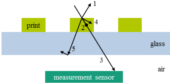
Figure 6: Schematic drawing of causes for differences between geometrical coverage and transmittance
