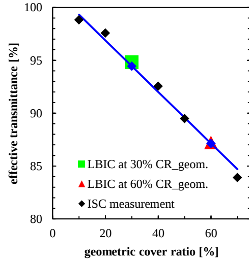
Figure 11: Calculation of the effective transmittance of printed front glass based on I_{SC} measurements on module samples with 30 and 60% coverage ratio versus measurements at other coverage ratios; effective transmittance calculated from LBIC measurements performed on samples with 30% (large green square) and 60% coverage ratio (large red triangle)
