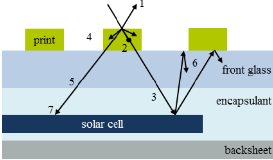
Figure 9: Schematic drawing of causes for differences between transmittance measurements and power measurements
