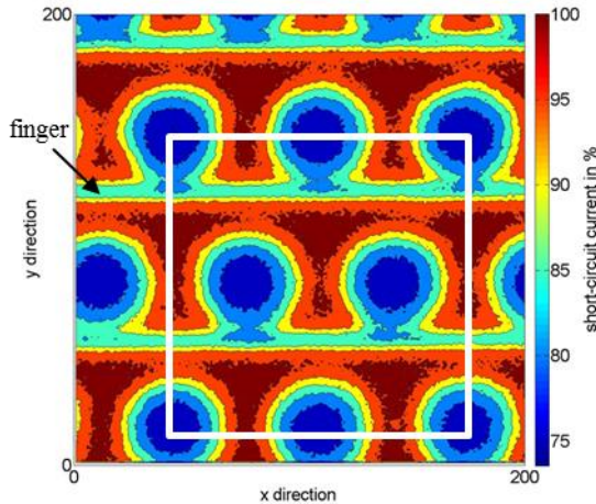
Figure 10: LBIC measurement results, spatially resolved relative short circuit current of a 1 mm white dot pattern. The area for spatial integration is outlined in white.
