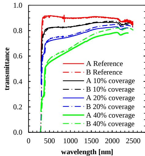
Figure 5: Transmittance spectra of glass samples covered with decorative elements (white dots), small (A) and large-area (B) illumination measurement setup, no additional weighting
