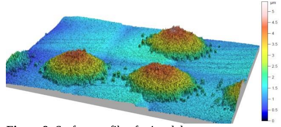
Figure 8: Surface profile of printed dots
