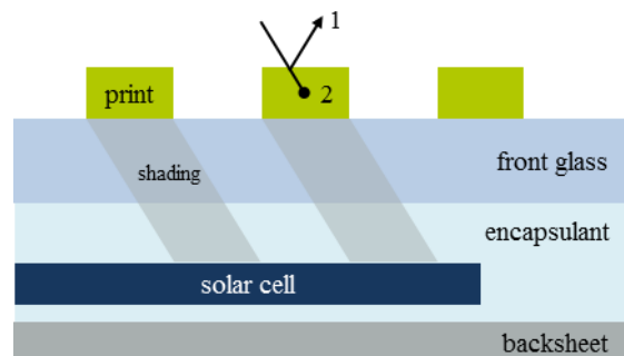
Figure 3: Schematic drawing of changes in module optics by application of decorative prints onto the module front cover
