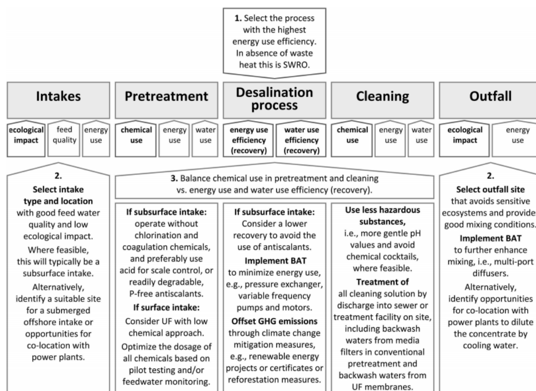
Figure 4: Roadmap to 'green' or 'sustainable' desalination (Figure 24 in Lattemann (2010))
