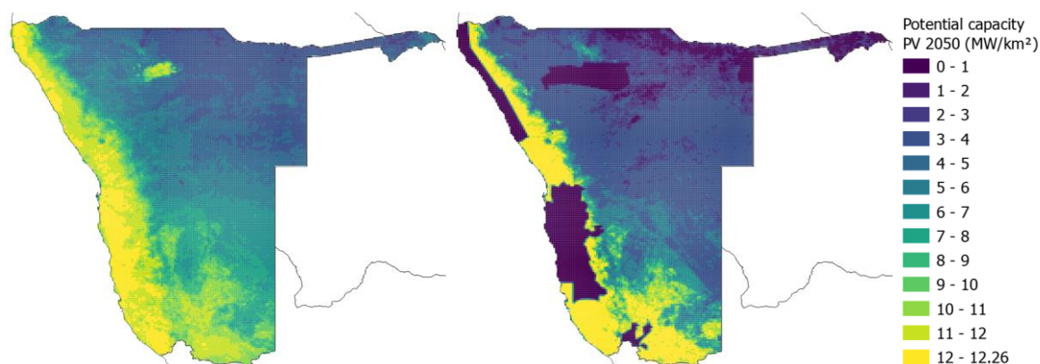
Figure 3: Potential PV capacity (in MW/km 2 ) in Namibia in 2050 without excluding protected areas (left) and excluding protected areas up to IUCN category II (right)
