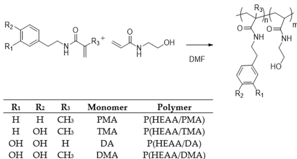
Figure 2. AIBN initiated polymerization with dopamine-modified acrylamides and HEAA to copolymers.
