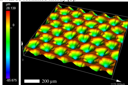
Figure 3: Glass surfaces were treated in a two-step process sequence using laser processing and wet chemical etching. An exemplary false-color image of the height profile of a periodic structure measured applying confocal microscopy is shown.
