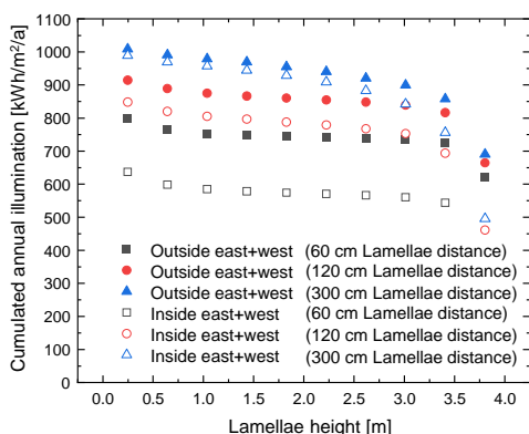
Figure 2: Top: Simulation results showing the cumulated annual light energy hitting different surface portions of a façade with differently spaced perpendicular PV lamellae in Germany.
