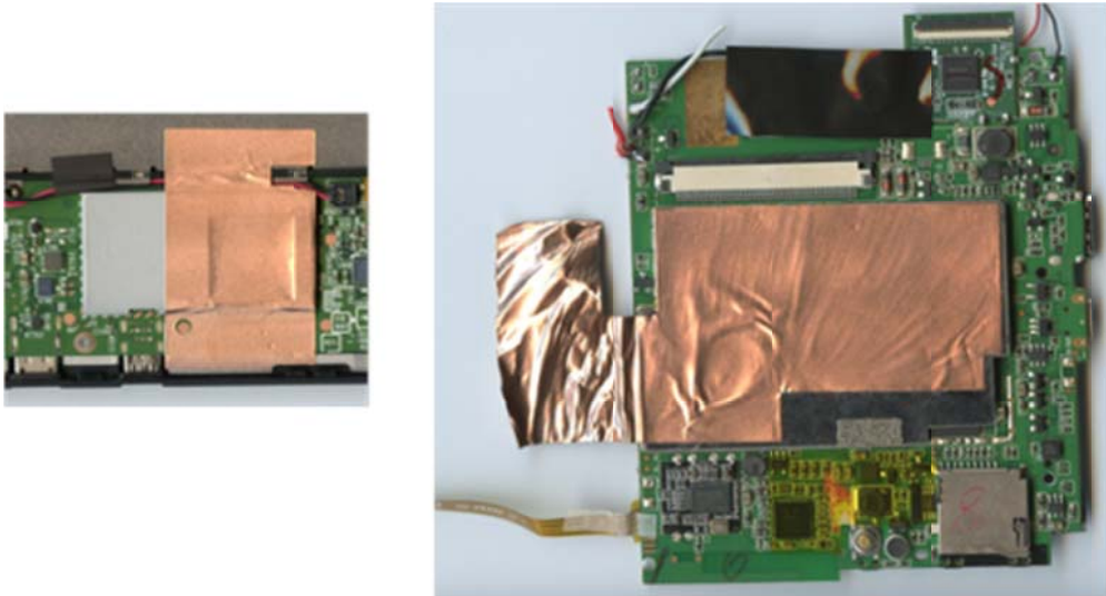
Figure 54: DUT_10 (left) and DUT_04 (right) with EMI-shields fixed with adhesive tape
