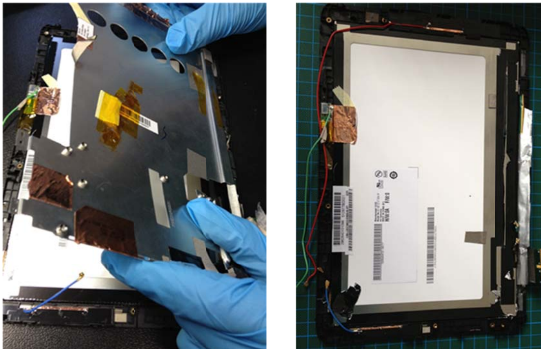
Figure 59: DUT_03 Take away the metal shield
