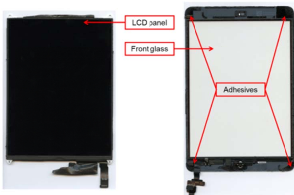
Figure 55: DUT_07 separation of front glass and LCD panel
