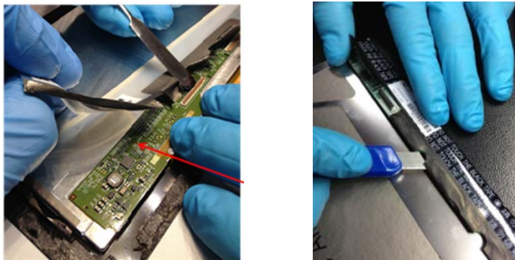
Figure 63: DUT_02 (left) and DUT_01 (right) taped over display driver board
