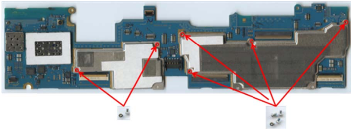
Figure 52: DUT_01 EMI shields connected with screws
