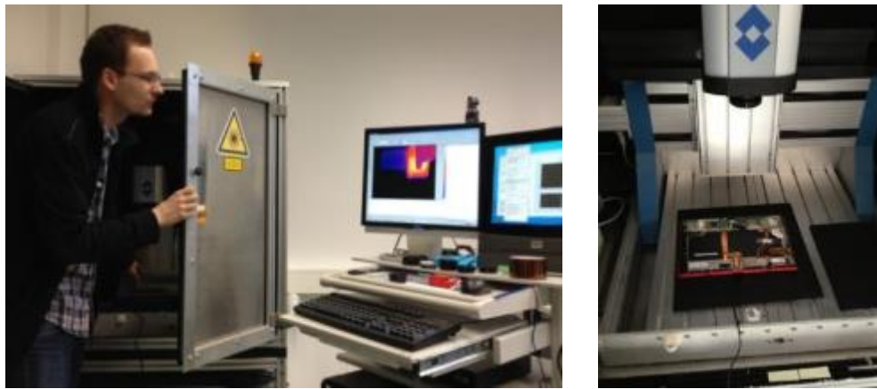
Figure 3: Thermography set-up
