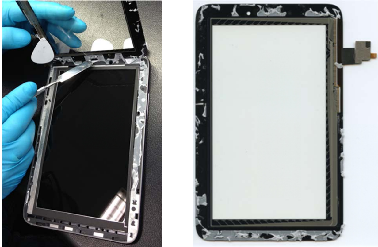
Figure 61: DUT_06 separation of front glass from display unit
