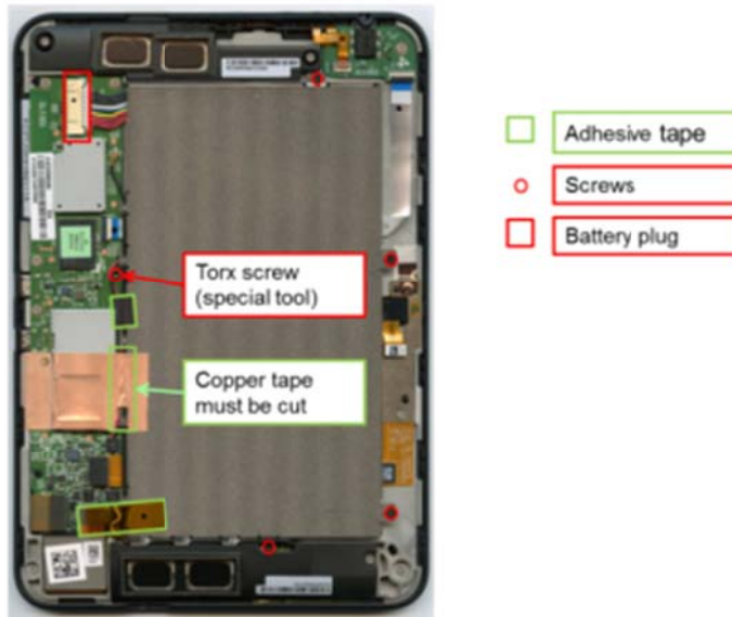
Figure 42: DUT_10 torx screws and problematic tapes
