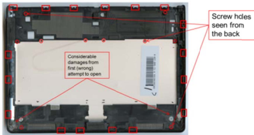
Figure 28: DUT_02 removal of back-cover
