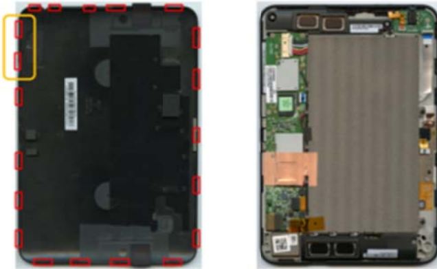
Figure 21: DUT_10 opening mechanism
