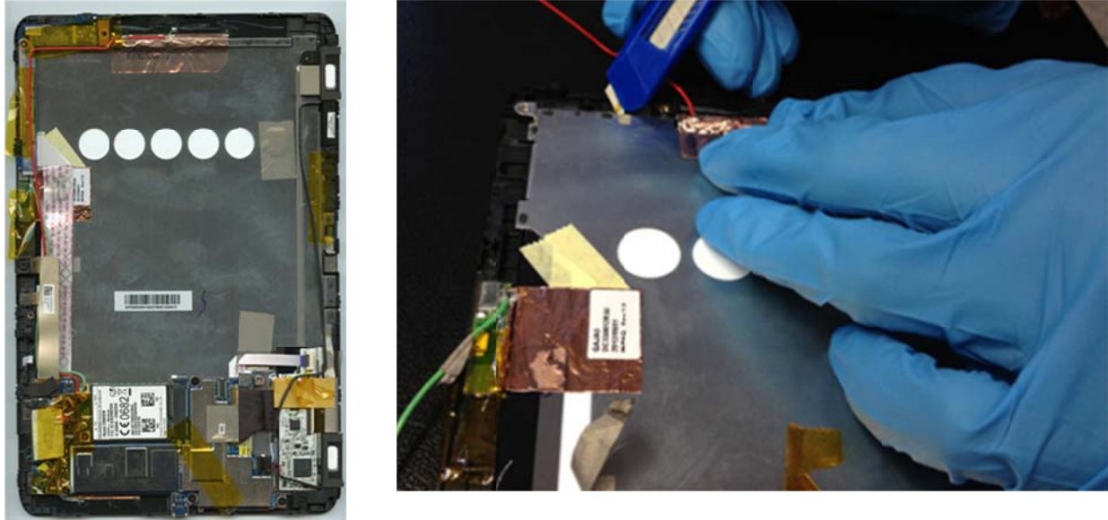
Figure 58: DUT_03 Cutting free the metal shield on the back-side of the display unit
