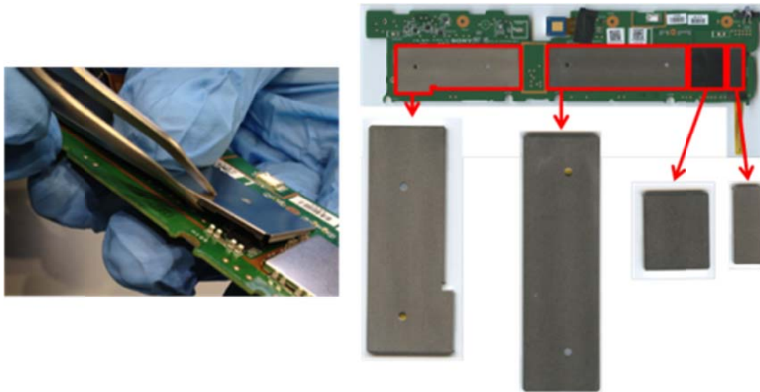
Figure 53: DUT_02 Clipped-on EMI-shields
