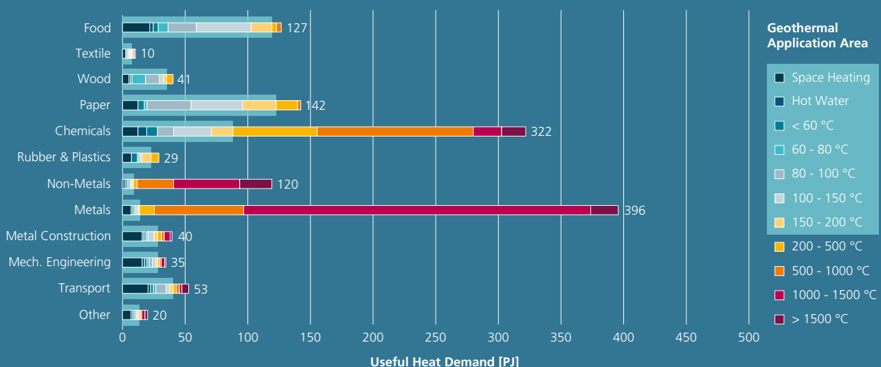
Figure 6: Sector-specific breakdown of useful heat demand by application and temperature level (3.6 PJ = 1 TWh) 37 . Geothermal sources in direct use or in combination with large-scale high-temperature heat pumps can cover the demand for useful heat up to 150 °C and in the medium term (up to 2030) up to 200 °C.
