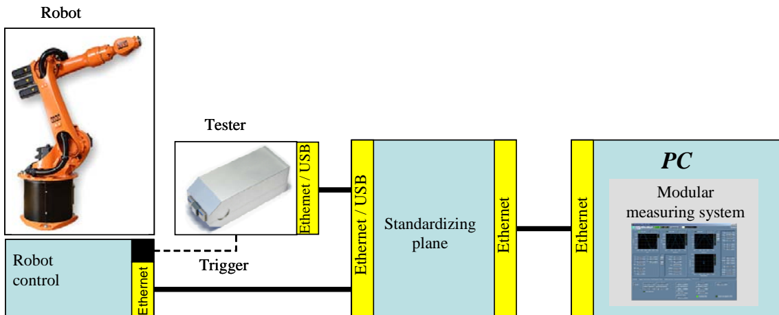
Figure 8. Modular Robotic Platform w/ Standardized Control Module
