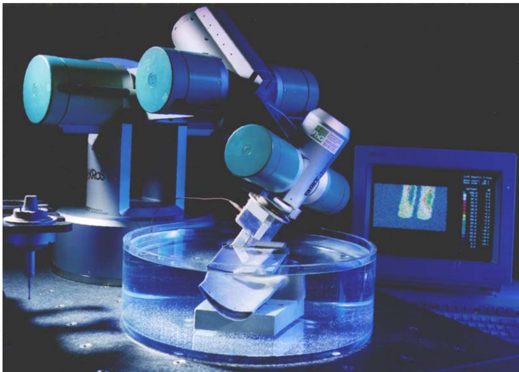
Figure 9. Ultrasonic Inspection of Freeform Surface Objects
