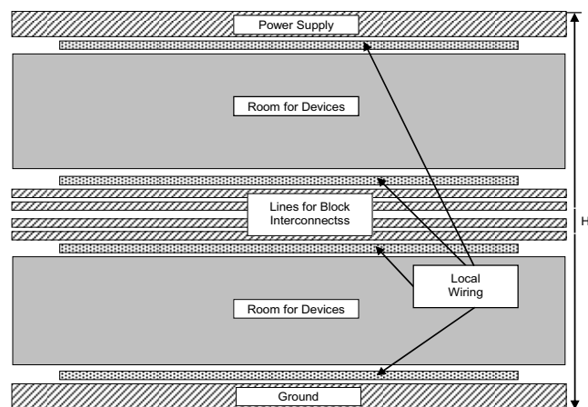
Figure 3. Street principle for layout floorplan
