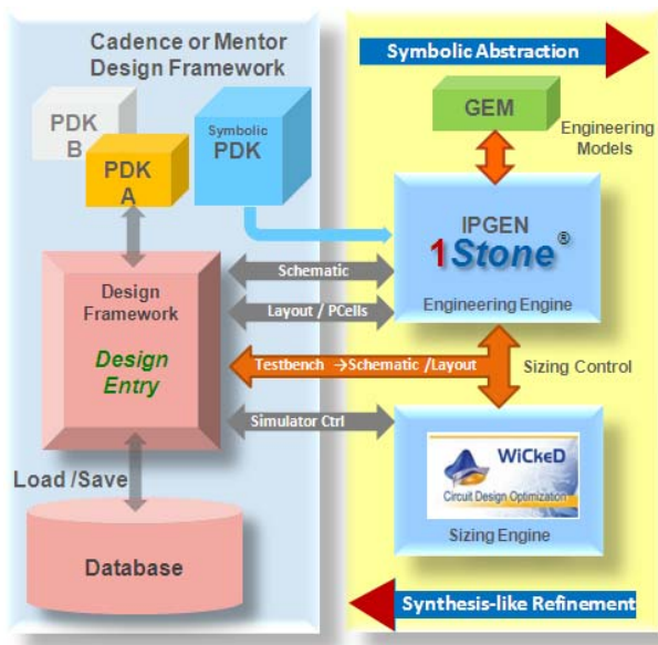
Figure 1. Design Flow Extension that enables analog IP Retargeting and Design Porting
