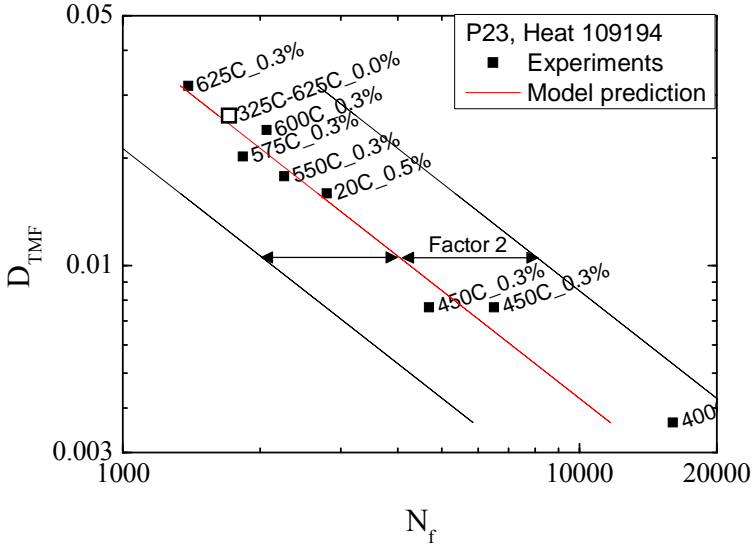
Figure 6: Experimental and predicted cycles to failure
