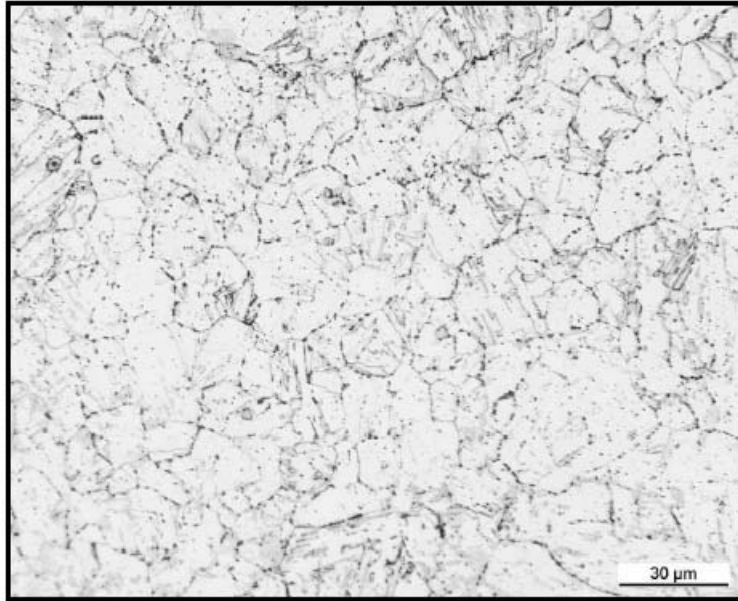
Figure 1: tempered bainitic microstructure of tubes ODxWT 88.9x17mm (mid-thickness)
