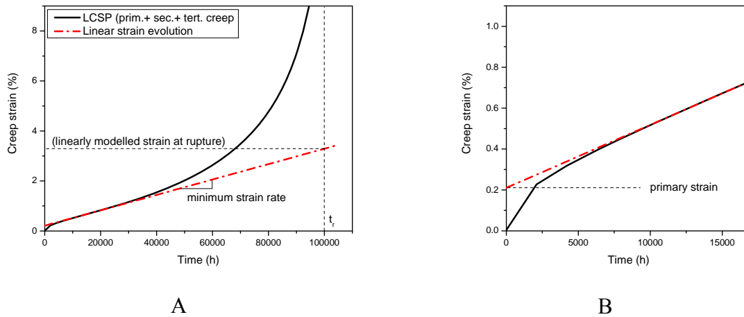
Figure 3: Creep strain prediction (LCSP and Norton type) for P23 at 575°C / 91 MPa (predicted rupture at 100 000 h); A: full creep curve, B: close-up on primary creep stage
