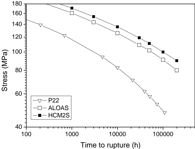
Figure 2: Intermediate creep rupture models at 575°C, for ALoAS P23 (open squares) in comparison to HCM2S (black squares, data from literature) and P22 (10CrMo9-10, according to EN-10216). ALoAS long term creep strength has been extrapolated.
