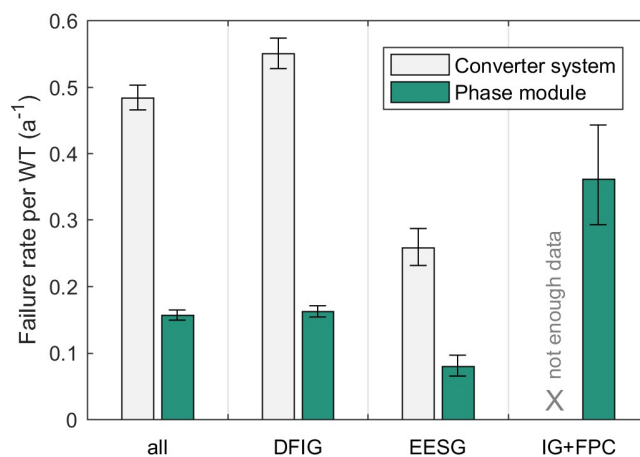
Fig. 6. Comparison of average failure rates of the overall converter system (left bar) and the phase-module components (right bar) as the core of the converter among wind-turbine groups with different generator-converter concepts
