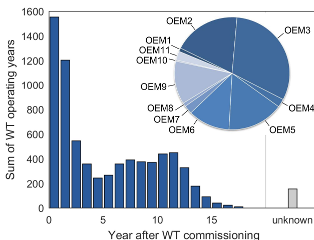
Fig. 3. Amount of evaluated data from wind turbines of different ages (bar chart) and portions of turbines by different manufacturers (pie chart, based on evaluated number of WT operating years)
