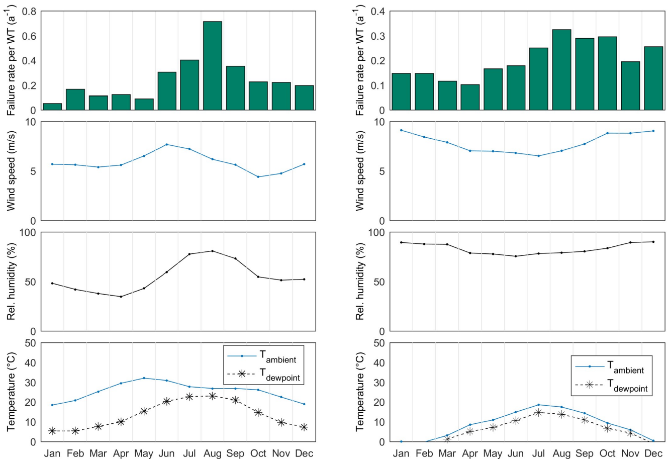
Fig. 10. Seasonal variation of phase-module failure rates in India (left, based on data from 590 WT operating years) and Scandinavia (right, 933 WT operating years) with corresponding monthly average values of wind speed, ambient temperature and relative humidity
