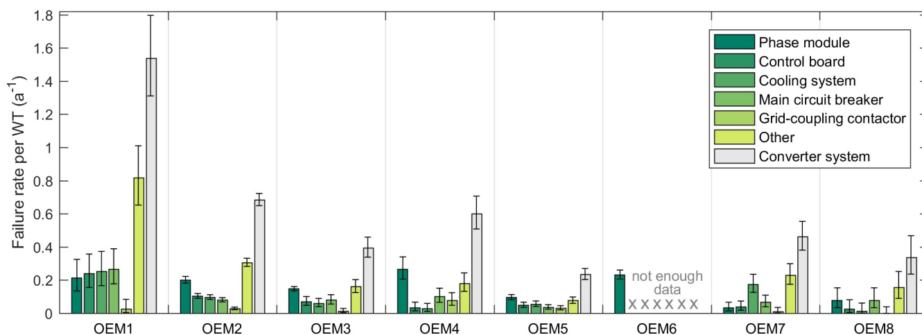
Fig. 7. Average failure rates of the overall converter system and its components in groups of DFIG-based wind turbines of manufacturers OEM1...OEM8
