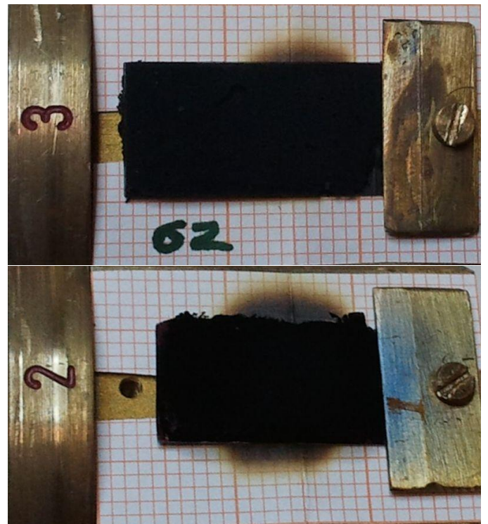
Fig. 4 Two of the samples (top: Ae_62/A-8, bottom: LP447a) after irradiation with 10^{17} p/cm 2 and 5 \times 10^{17} p/cm 2 , respectively.
