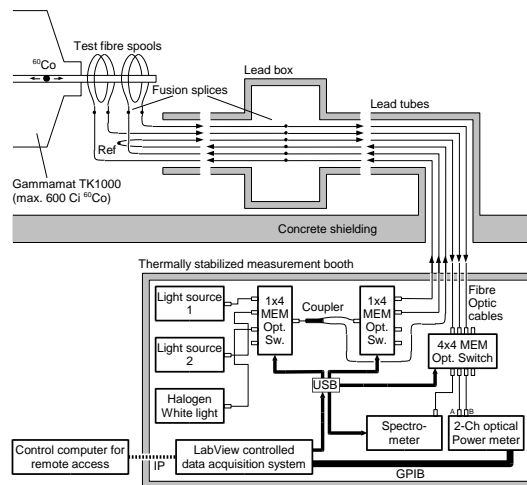
Fig. 1. Experimental Setup for optical fibers irradiation test using a ^{60}\text{Co} source
