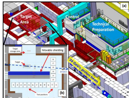
Fig 8. (a) 3D view of the facility and (b) a horizontal cut of the inner target chamber. Racks 1 to 18 are the regions representing the test locations. The blue, grey and brown plates are respectively iron, concrete and marbles blocks.
