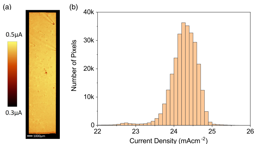
Figure 2. a) Image of LBIC data of the record 1.1 cm 2 organic solar cell. b) Histogram showing the distribution of the current density normalized to the value of J_{SC} under “1 sun” (global AM1.5).
