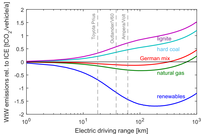
Figure 4 Well-to-wheel (WtW) CO 2 emissions in tonnes per vehicle and year for PHEV as compared to a conventional vehicle versus all electric ranges (AERs) for different electricity types (blue: renewable energies; green: natural gas; red: German mix; cyan: hard coal; purple: lignite). CO 2 = carbon dioxide; km = kilometers; PHEV = plug-in hybrid electric vehicles; rel. to ICE = relative to internal combustion engine; tCO 2 /vehicle/a = tonnes of carbon dioxide per vehicle per annum.
