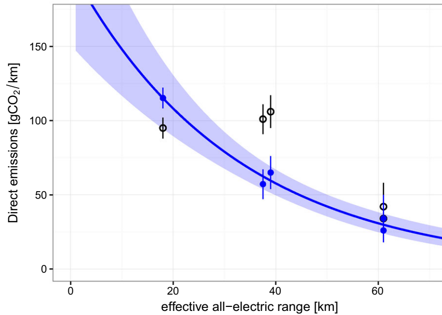
Figure 2 Direct CO 2 emissions of PHEVs with different all electric ranges (AERs). The average specific CO 2 emissions of the five PHEV models are shown as observed in our sample (empty symbols) and adjusted for their different propulsion system powers (filled symbols) with regression result (solid line). The blue bands indicate 95% confidence bands. CO 2 = carbon dioxide; gCO 2 /km = grams of carbon dioxide per kilometer; PHEVs = plug-in hybrid electric vehicles.
