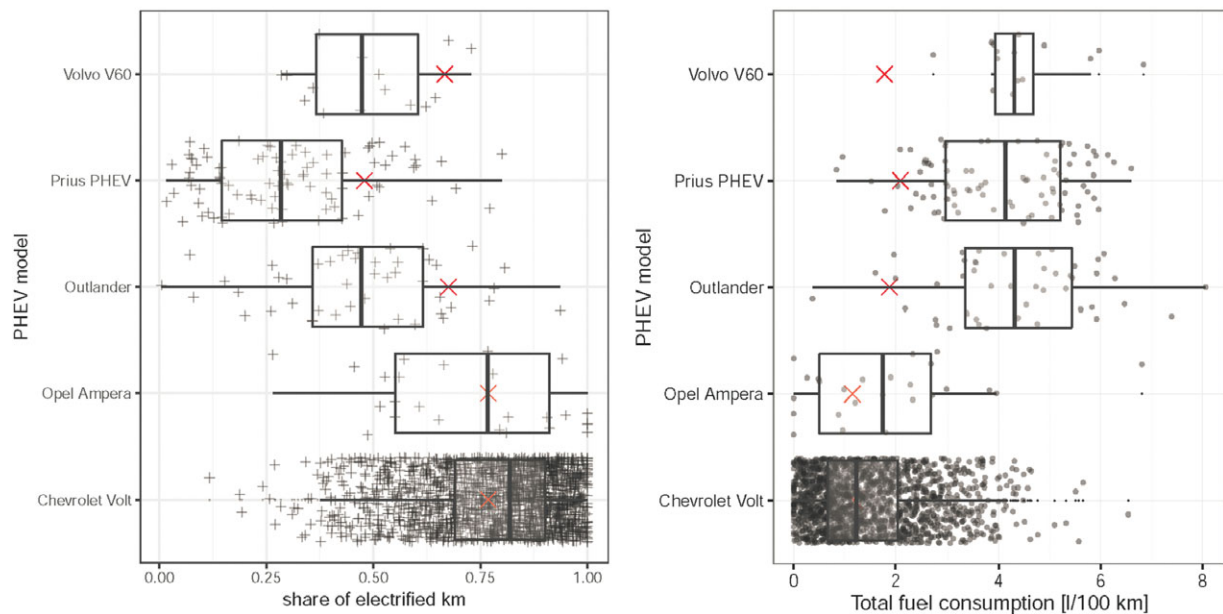
Figure 1 Fuel consumption of PHEVs. Shown are empirical individual values (small dots) and box plots for the five PHEV models. The left panel shows the share of electrified kilometers, that is, the utility factor (UF). The right panel shows the fuel consumption in liters per 100 kilometers (l/100km). The crosses indicate official driving cycle values. PHEVs = plug-in hybrid electric vehicles.
