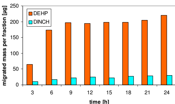
Figure 1: Mass plasticiser migrated into enteral feeding solution per 3 hours (15 ml fraction) at room temperature and a flow rate of 5 \text{ ml h}^{-1} (realistic application conditions)
