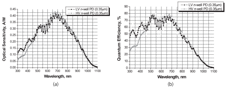
Figure 3: (a) Optical sensitivity curves (average) obtained from LV n -well PD and HV n -well PD photodetector structures fabricated in the 0.35 \mu m CMOS process available at the Fraunhofer IMS; (b) quantum efficiency average curves obtained for (a) [4].
