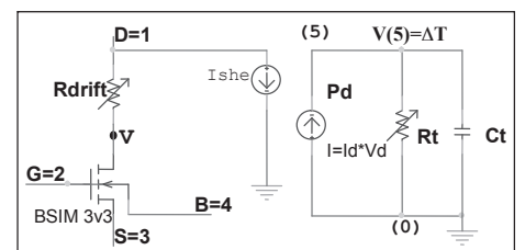
Figure 4: Modeling the self-heating effect.
