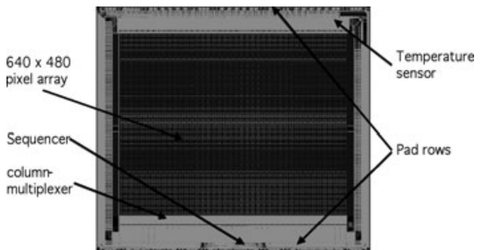
Figure 6: Layout IRPGA with 640 x 480 pixel digital readout
