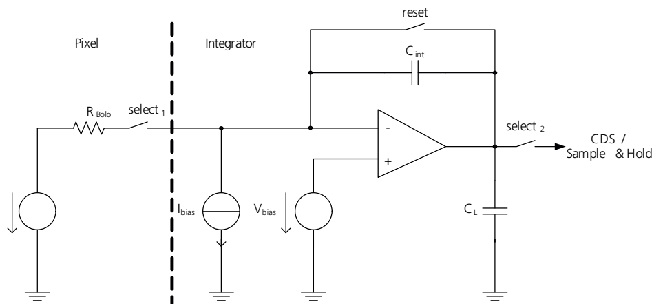
Figure 3: Analog readout principle: Integrator
