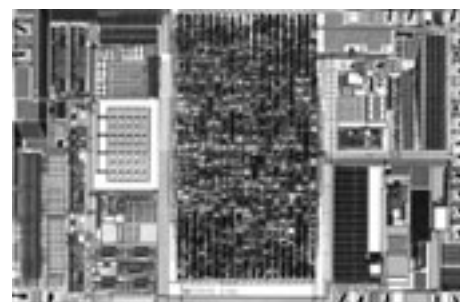
Figure 2: IMS SoC solution for wireless pressure sensing
