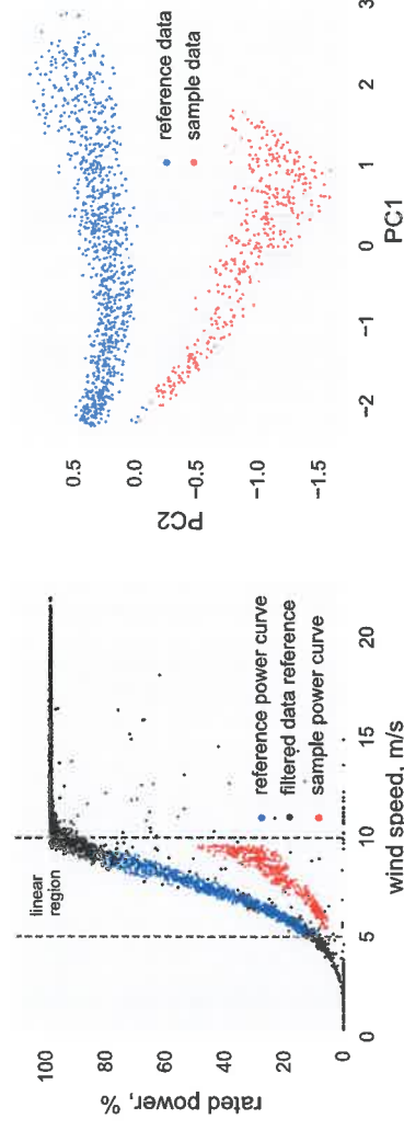
(a) Data-preprocessing.
