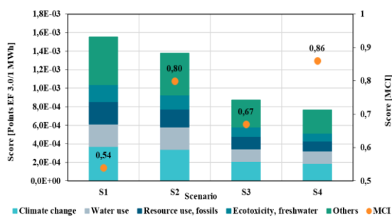
Figure 1: Normalized and weighted single score results (EF3.0) of environmental impacts by category
