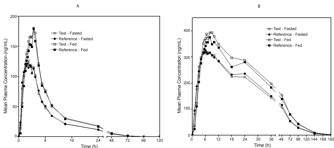
Figure 2: Mean bupropion and hydroxybupropion plasma concentration vs. time curve. A single oral dose administration of 150 mg bupropion tablet formulation (test or reference Zyban®) was given to 78 volunteers divided in two groups. Group 1 was composed of 42 subjects (21 men and 21 female) and received the bupropion tablet without any special meal prior the drug administration. Group 2 was composed of 36 subjects (18 men and 18 female) and received the bupropion tablet after taken a hyperlipemic meal prior the drug administration. Panel (A) shows the bupropion plasma concentrations and panel (B) shows the hydroxybupropion plasma concentrations.
