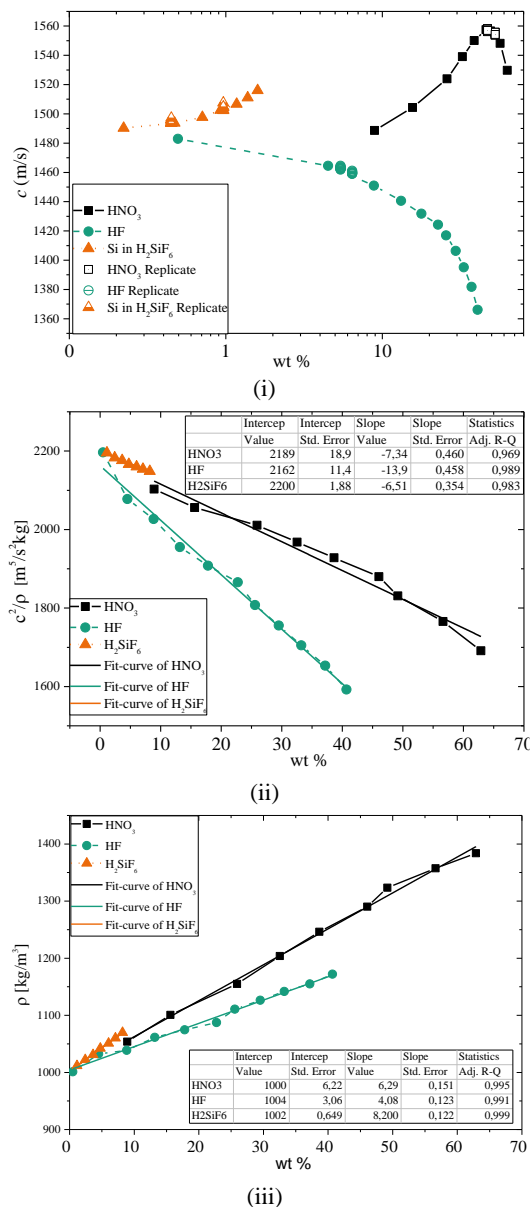
Figure 2: Sound velocity (i), bulk modulus (ii) and density (iii) of individual acids as a function of the concentration in weight percent.
