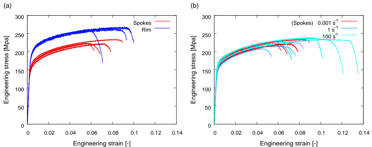
Fig.5: Engineering stress vs. engineering strain with regard to location for quasi-static tensile tests (a) and strain rate for specimens from the spokes (b).
