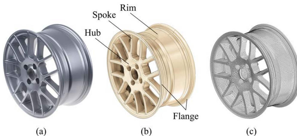
Fig.1: Reverse engineering process, (a) real wheel, (b) CAD model, (c) FEM model.
