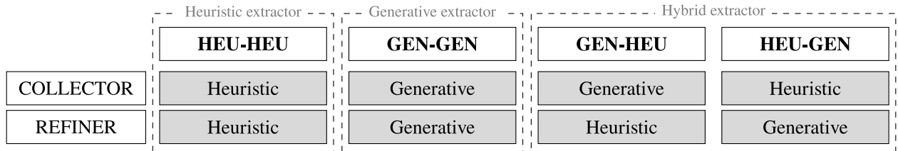
Fig. 3. Four extractor variants.
