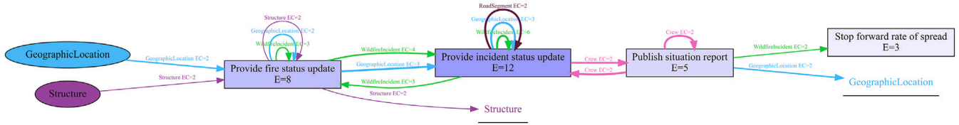
Fig. 9. OCDFG based on an OCEL derived with the GEN-GEN extractor variant for fire status updates regarding the Lilac Fire in January 2025 in San Diego.
