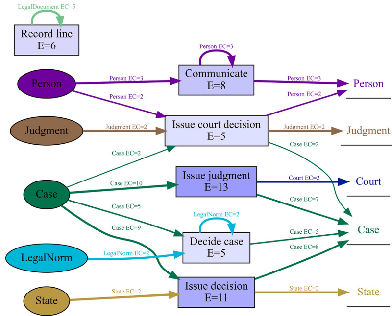
Fig. 11. ODFG based on an OCEL derived with the GEN-GEN extractor variant for the legal judgment of F.S.M. v. Spain.
