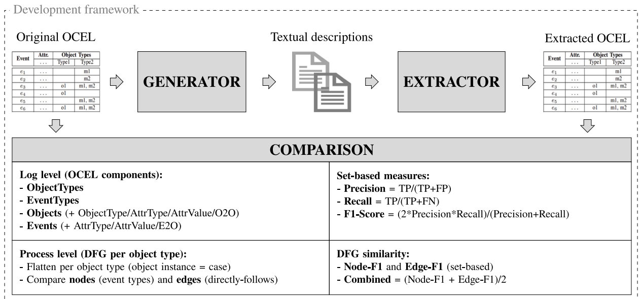
Fig. 4. Development framework.
