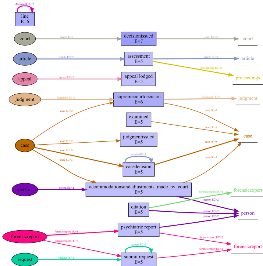
Fig. 12. ODFG based on an OCEL derived with the GEN-HEU extractor variant for the legal judgment of F.S.M. v. Spain.
