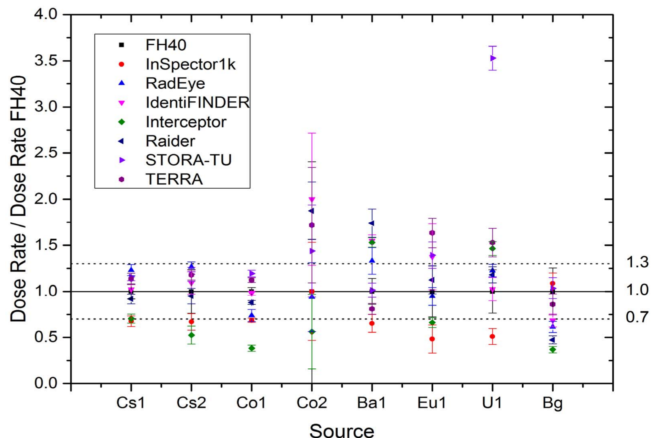
Fig. 3: Dose rate results for different detection systems depending on used sources
