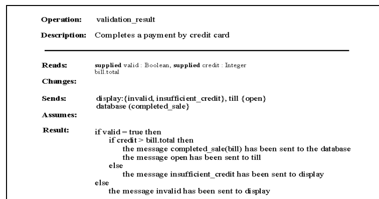
Figure 5: Operation Schema
