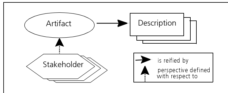
Figure 2: Artifact-oriented Approach
