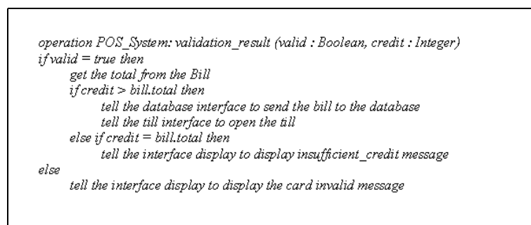
Figure 8: Operation Pseudocode
