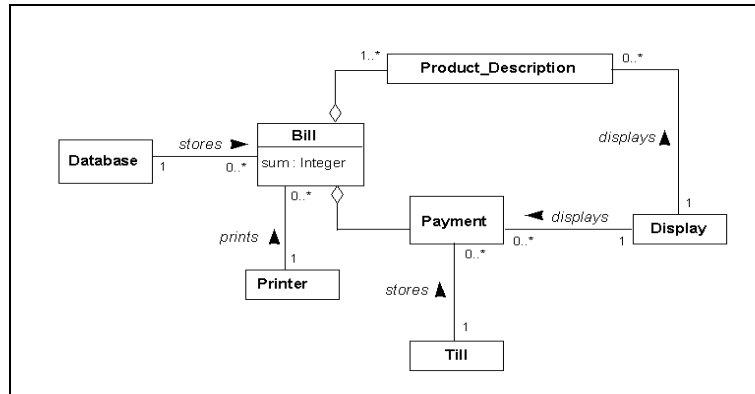
Figure 6: Class Diagram
