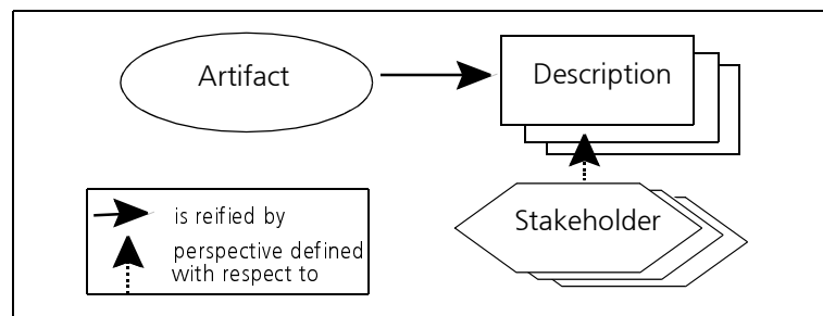
Figure 3: Description-oriented Approach
