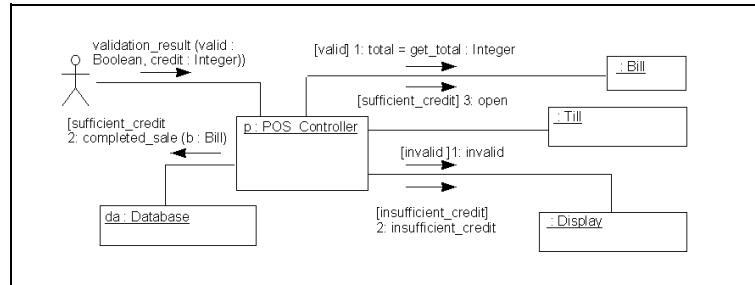
Figure 7: Collaboration Diagram
