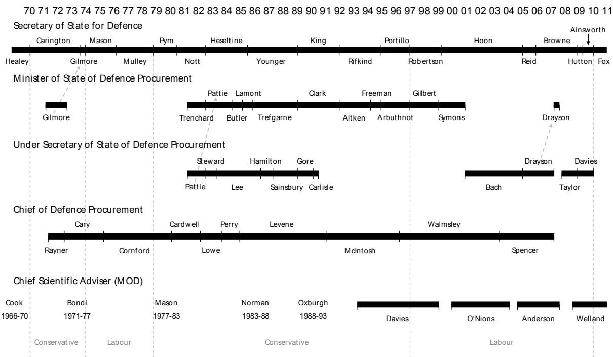
Figure 1: MOD stakeholders in defence related R&D
