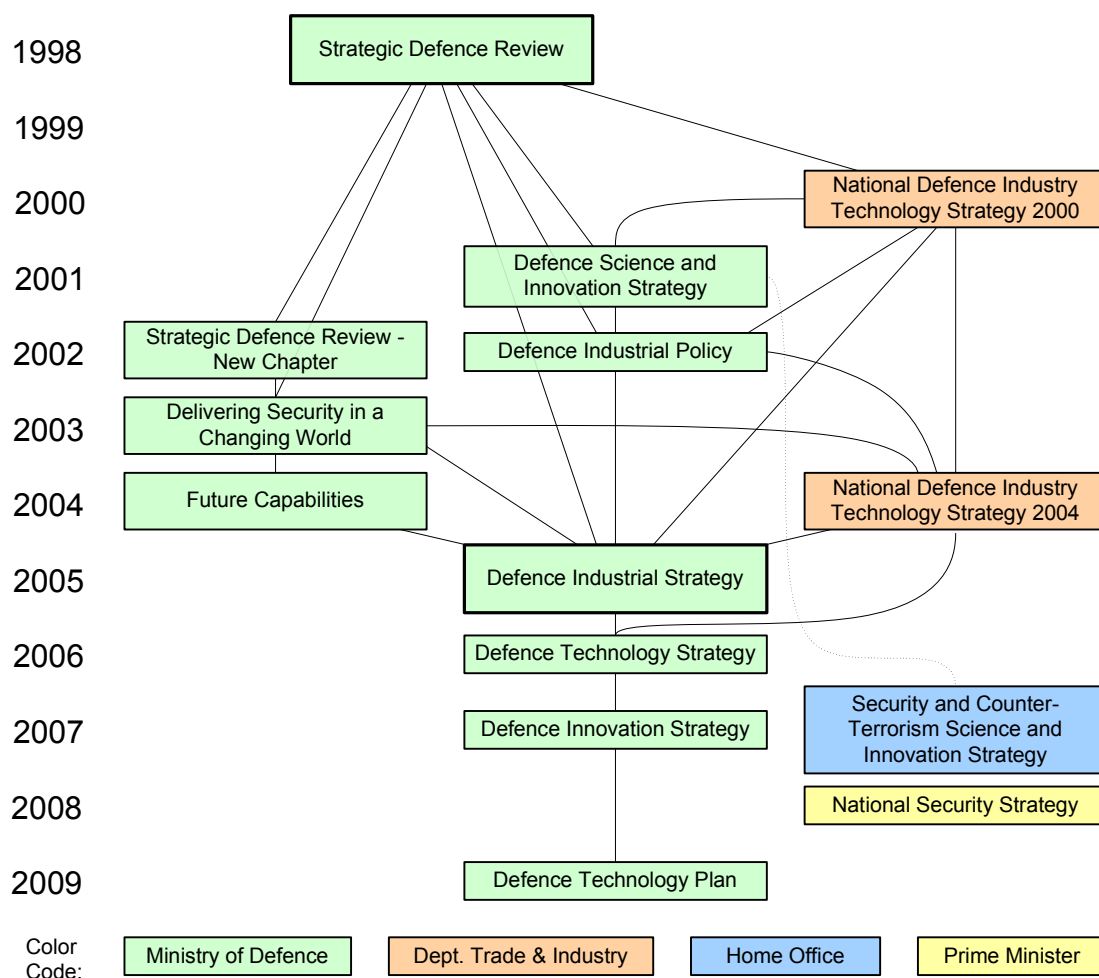
Figure 3: Relation of British doctrinal publications since 1998
