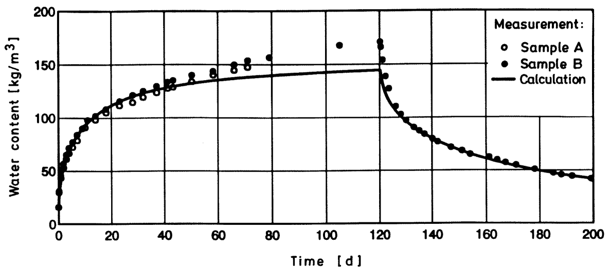
Fig. 42 Comparison between the measured and calculated mean water contents of the test piece during the suction process and during drying which begins after 120 days by removal of the water container. Sample A was cut into slices after 72 days of the experiment, to determine the moisture distribution.
