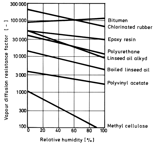
Fig. 18 Moisture dependence of the water vapour diffusion resistance factor of different organic building materials and coatings, according to [61]
