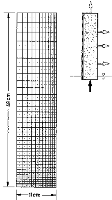
Fig. 41: Diagram showing the numerical grid for the two-dimensional calculation of the moisture process in the masonry stone test piece. The points in the middle of the grid elements represent the variable positions.
