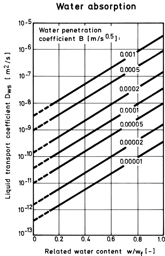
Fig. 21 Dependence of the capillary transport coefficient for the suction process on the water content and the water penetration coefficient of the building material, determined by means of the approximation relation in equation (24).
