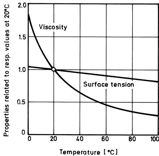
Fig. 14 Change in viscosity and surface tension of a water as a function of temperature, related to the values at 20°C, according to [21].
