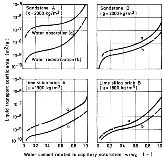
Fig. 15 Moisture transport coefficient of our different building stones as a function of the standardized water content [65]. The difference between the coefficients for capillary suction in contact with water (a) and redistribution after interruption of the water supply (b) is considerably greater in natural stone A (coarse pores) than in natural stone B (fine pores). In the case of lime silica brick, too, there are differences in transport coefficients which are based on density or production, but these differences are less pronounced.
