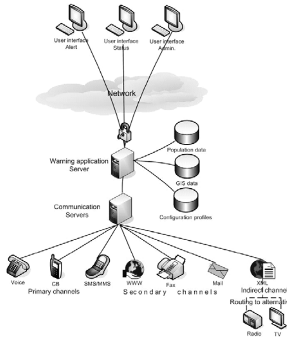
Figure 3: Telecom-based warning system. Source: UMS company (Norway). Website: http://www.umscom.com/
