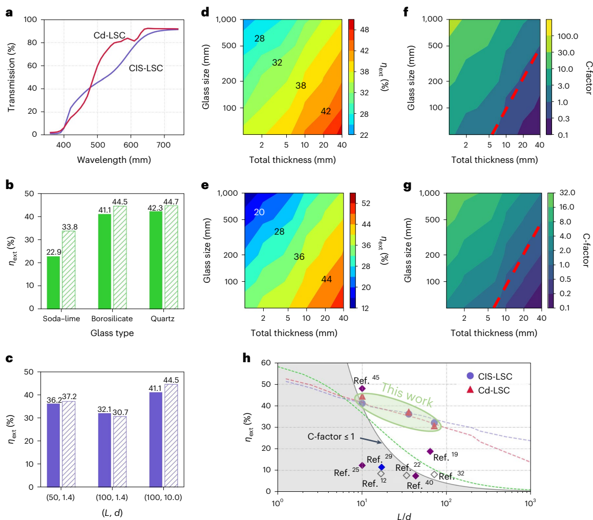
Fig. 2 | Experimental and simulation results of LSCs. a , Transmission spectra of CIS-LSC (blue) and Cd-LSC (red). b , Glass-type-dependent \eta_{\text{ext}} ( L, d = (100 \text{ mm}, 10 \text{ mm}) ). c , \eta_{\text{ext}} at different ( L, d ) values (in mm). For b and c , the filled boxes are CIS-LSCs and the dashed boxes are Cd-LSCs. d, e , Calculated \eta_{\text{ext}} of CIS-LSC ( d ) and Cd-LSC ( e ). f, g , Calculated C-factor of CIS-LSC ( f ) and Cd-LSC ( g ). The red dashed lines are guides for C-factor \cong 1 . In d–g , each data point presents the average value from 40,000 MC simulations. h , Experimental
