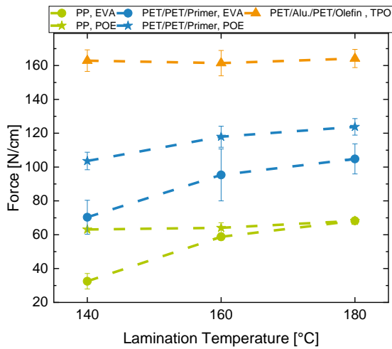
Figure 6: Initial peel forces obtained from the glass-encapsulant interface
