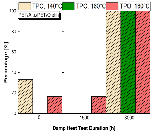
Figure 5: Failure type distribution of the different material combinations
