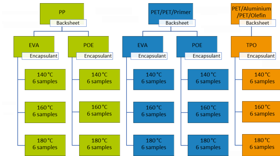
Figure 2: Material combinations and number of laminates built for the study
