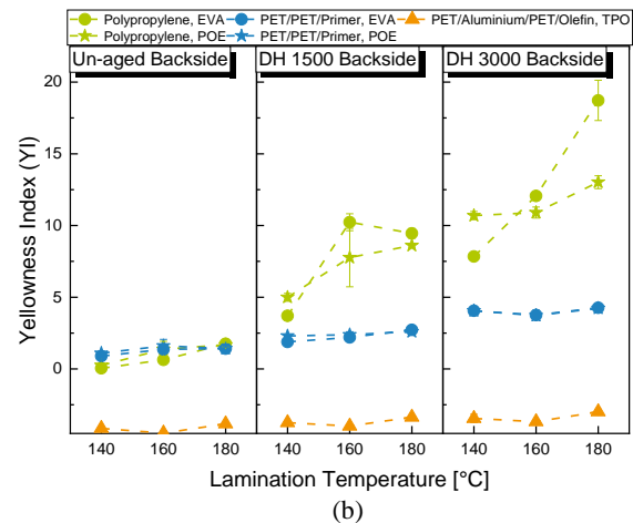
Figure 8: Yellowness index of the laminates with different material combinations (blue, green, orange) at different peak lamination temperatures on the (a) front side and (b) rear side of the laminate after lamination (left), after DH 1500 (middle), and after DH 3000
