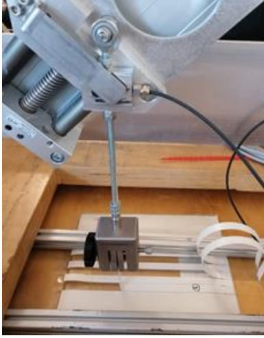
Figure 1: 90° Peel test at the glass-encapsulant interface
