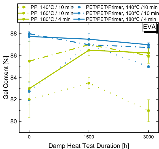
Figure 3: Gel-content of the EVA laminates with PP or with PET backsheet directly after lamination, after 1500 h and 3000 h damp heat test.
