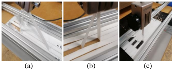
Figure 4: Photograph of the back sheet failure mode occurred during the peel test: Delamination of Backsheet in Sub-Layers (a), Delamination at the backsheet-encapsulant interface (b), and rupture of the Backsheet (c)
