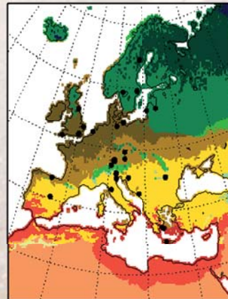
Climate for Culture Baseline 1960-1989 (Left) Far Future 2070-2090 (Right) T and RH.
