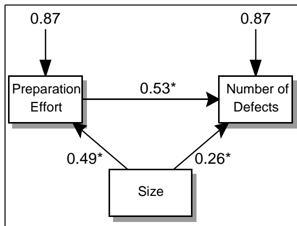
Figure 11: Path Diagram for Design Reviews
