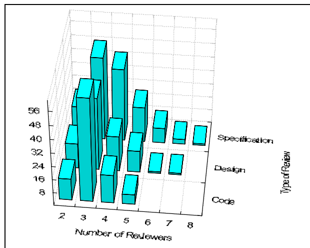
Figure 8: Histogram of the Number of Review- ers for the Different Types of Reviews
