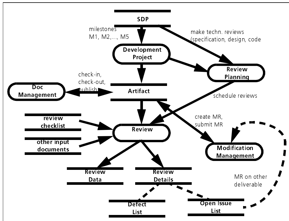
Figure 3: The Review Procedure at PRC-ON
