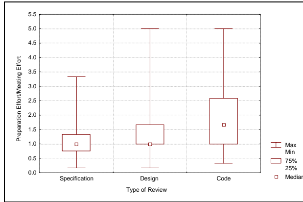
Figure 6: Relationship of Preparation Effort and Meeting Effort
