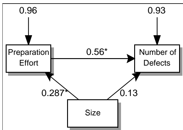
Figure 12: Path Diagram for Code Reviews
