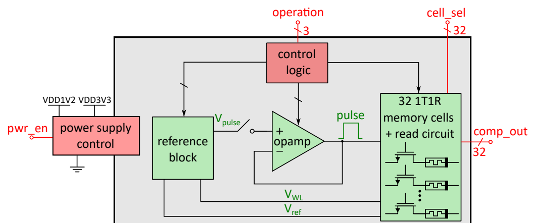
Figure 6. Block diagram of an RRAM memory block containing 32 1T1R memory cells and the necessary peripheral circuitry for reading and writing the cells [29].
