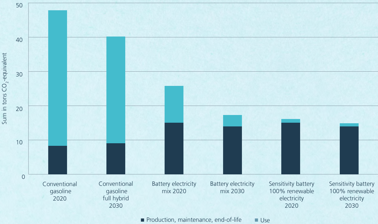
Figure 4 Greenhouse gas emissions from battery electric cars compared to conventional cars (compact class) over the entire life cycle for Germany for cars purchased in 2020 or 2030 [28]
