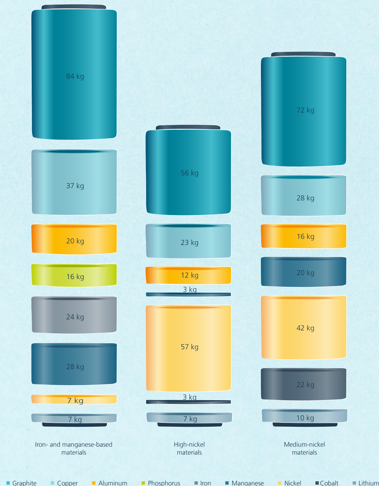
Figure 5 Average raw material requirements of a lithium-ion battery (gross capacity: 80 kWh) for different clusters of battery chemistries, in kilograms, excluding the demand for electrolytes and binders. [own, averaged calculation according to Fraunhofer ISI eEV database]
