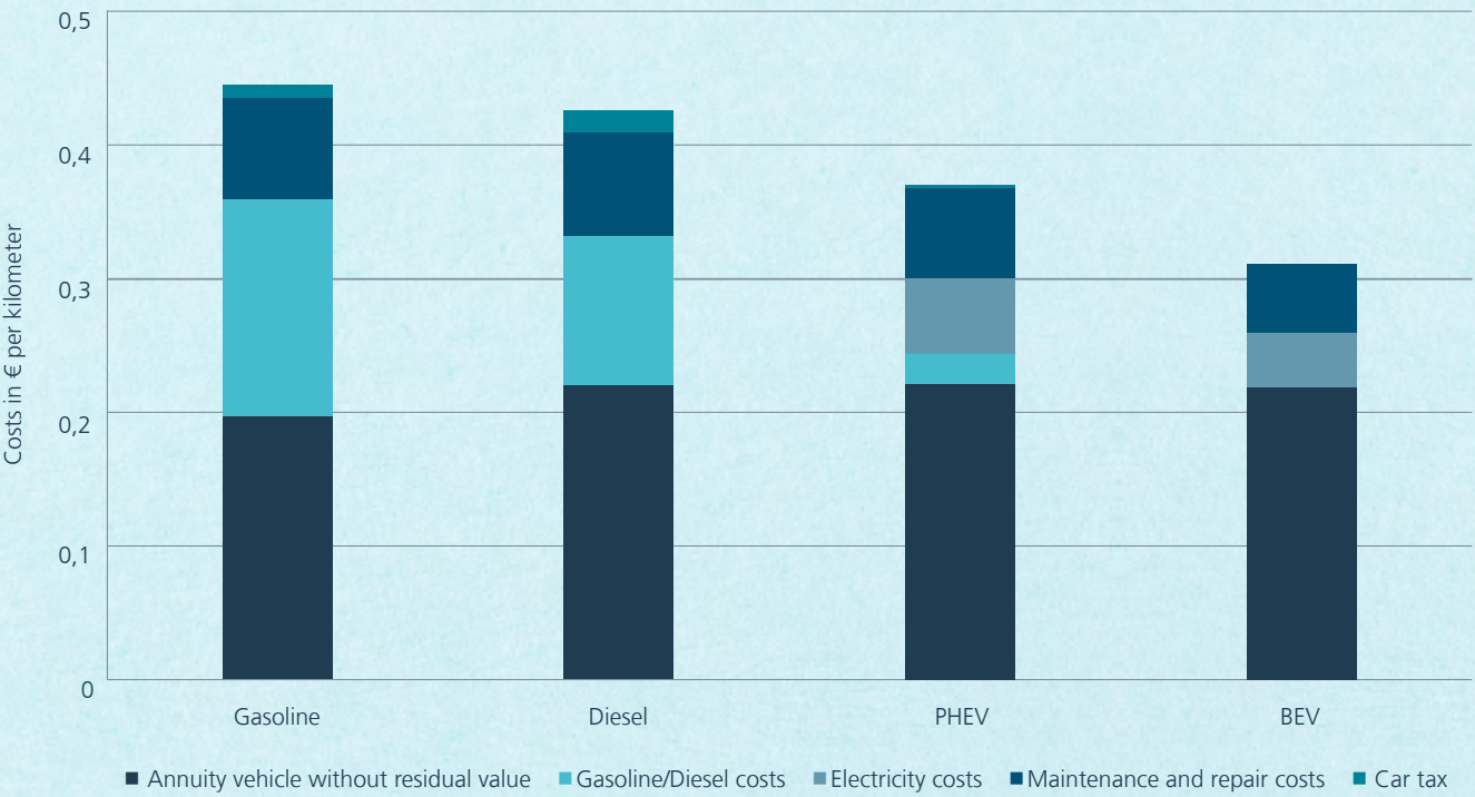
Figure 3 Comparison of the economic efficiency of conventional mid-range cars with battery electric vehicles (BEVs) and plug-in hybrids (PHEVs) in 2025 (source: Own representation based on [4])
