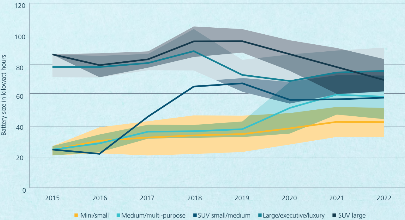
Figure 6 Average sales-weighted battery capacity in Europe from 2015 to 2022 shown by segment. The coloring indicates standard deviation. Own illustration, based on [44]
