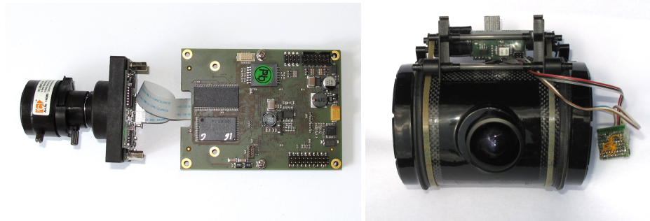
Fig. 3. A „smart“ camera (left) controls the UAV and is carried as a payload (right)
