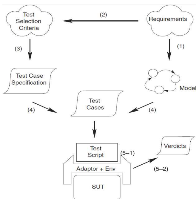
Figure 39: MBT Process
