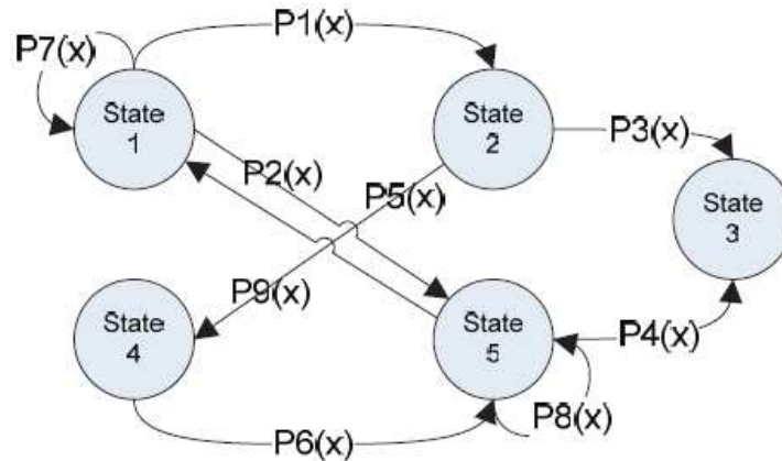
Figure 33 Markov model
