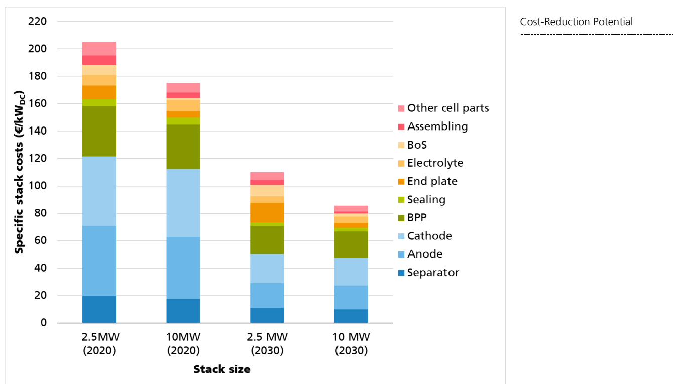
Figure 4-1: Comparison of specific next generation alkaline electrolysis stack costs for 2.5 MW and 10 MW stack sizes.
