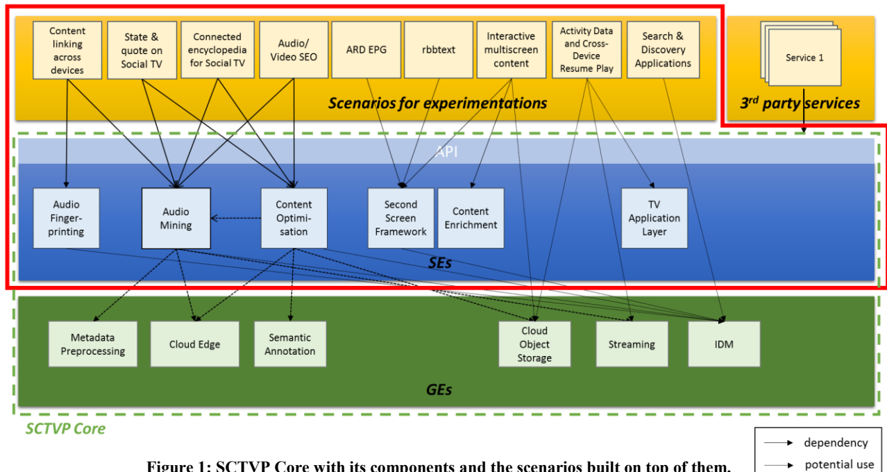
Figure 1: SCTVP Core with its components and the scenarios built on top of them.
