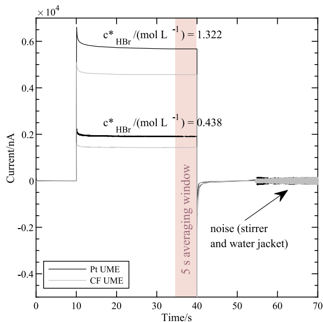
Fig. 3. Chronoamperometric transients of bromide oxidation currents (Experiment A) recorded at Pt and CF UMEs in 1.322 and 0.438 \text{ mol L}^{-1} HBr at 25^\circ\text{C} . The noise is visible after the stirrer and water flow in the water jacket have been switched back on.
