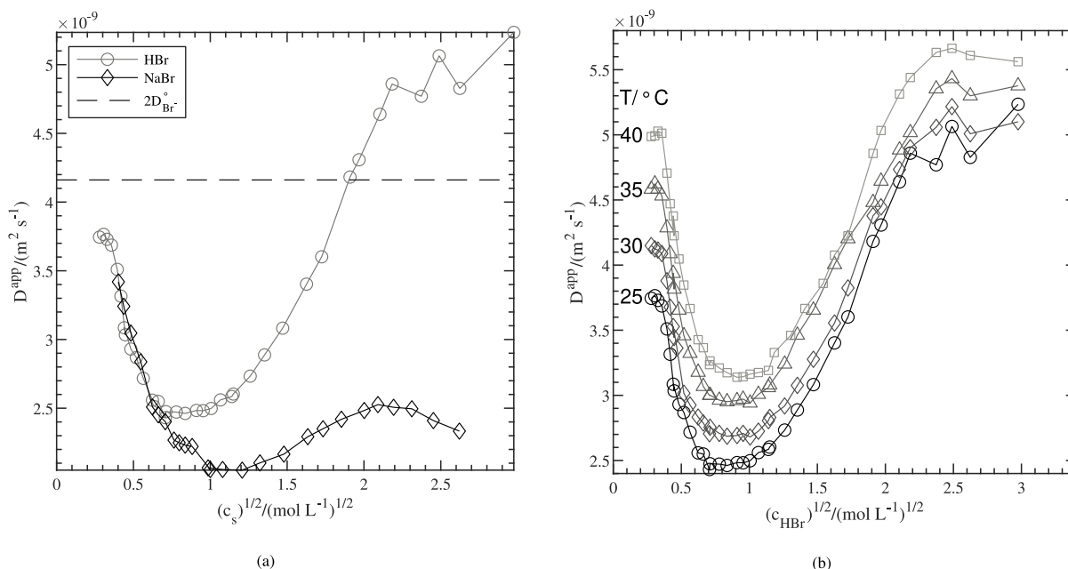
Fig. 5. (a) Apparent diffusion coefficients of bromide anions in HBr and NaBr aqueous solutions (mean from the Pt and CF UME experiments) at 25 °C. The limiting value of 2D_{Br^-}^\circ (factor of 2 due to migration contribution) is plotted for reference.; (b) Apparent diffusion coefficients of bromide anions in HBr solutions (mean from the Pt and CF UME experiments) at four temperatures between 25 and 40 °C. Lines connecting the experimental data points serve as a guide for the eye only.
