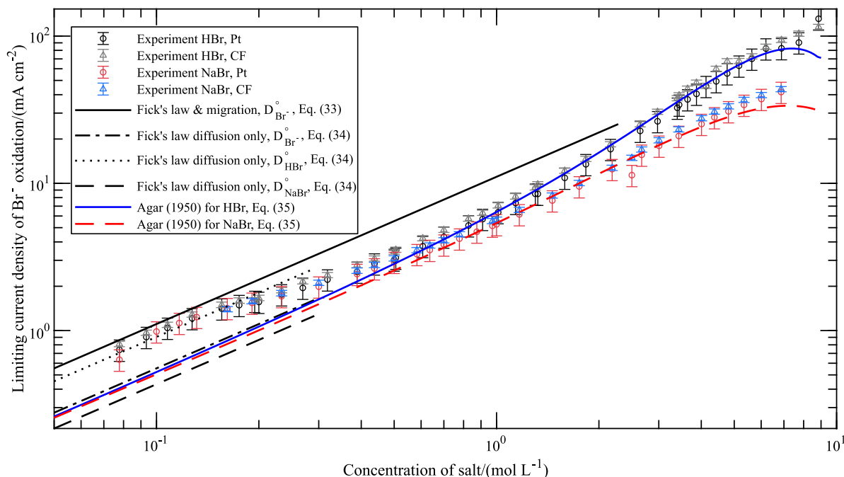
Fig. 4. Limiting current densities of the oxidation of bromide ions in HBr and NaBr solutions (Pt and CF UME experiments) at 25 °C. The modelling curves assuming D_{Br^-}^\circ (with and without the migration contribution) and ambipolar diffusion coefficients are plotted for reference. The experimental i_{lim} at CF UME were scaled (divided) by the electrode diameter ratio R_{el} = 1.44 to facilitate the comparison with Pt UME results.
