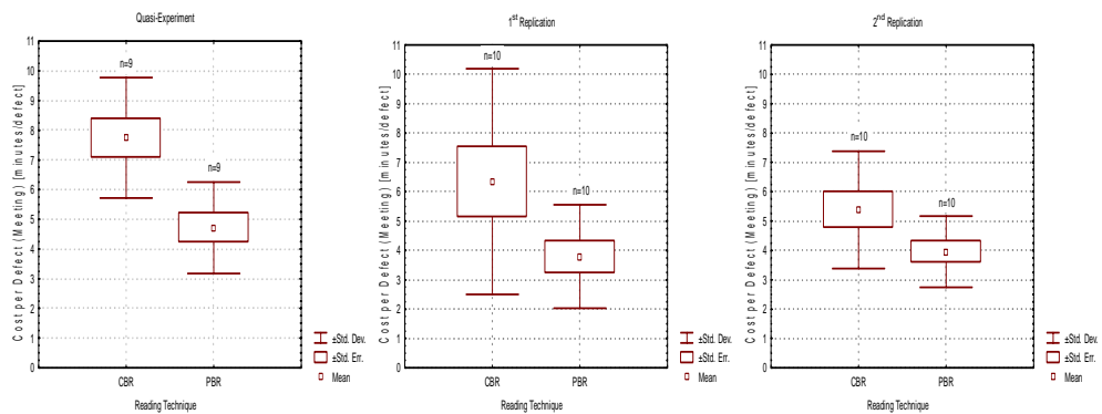
Figure 6: Box-Plots of the Cost per Defect for the Meeting Phase.
