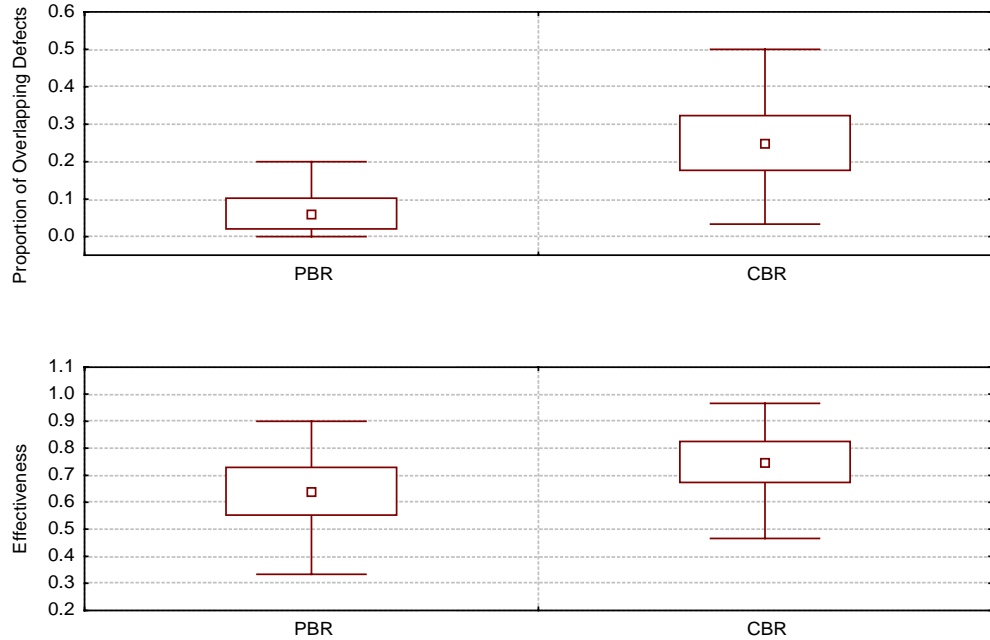
Figure 14: Results of a simulated inspection with PHIGH = 0.6 and PLOW = 0.1.
