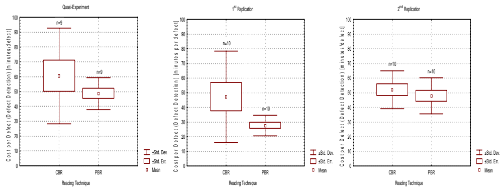
Figure 5: Box-Plots of the Cost per Defect Ratio for the Defect Detection Phase.
