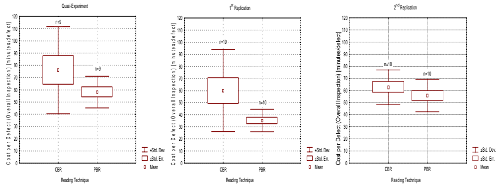
Figure 8: Box-Plots of the Overall Cost per Defect.
