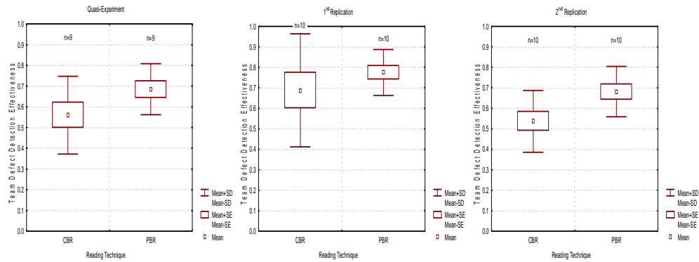
Figure 4: Box-Plots of the Team Defect Detection Effectiveness.23
