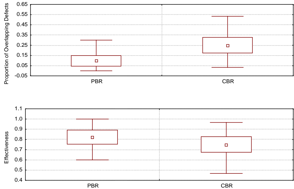
Figure 13: Results of a simulated inspection with P_{HIGH} = 0.8 and P_{LOW} = 0.12 .
