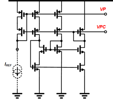
Figure 5. Unity current source. VP and VPC are used for current replica to unary and binary current elements.
