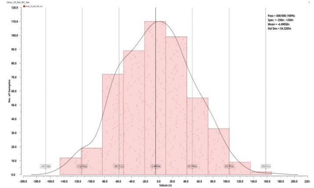
Figure 6. Monte-Carlo simulation result of the unary current source
