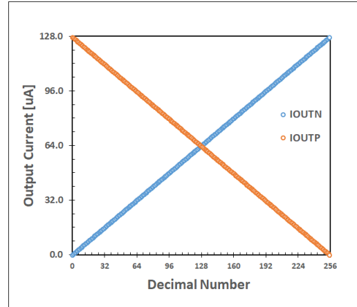
Figure 9. 8 bit full-scale output current of the CS-DAC
