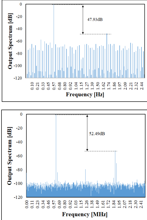
Figure 10. SFDR of the CS-DAC at 8 bit resolution (left) and at 12 bit resolution (right)
