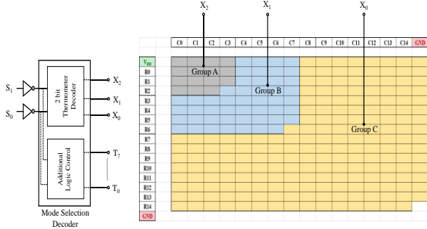
Figure 3. Conceptual view of the programmable 2-D unary matrix
