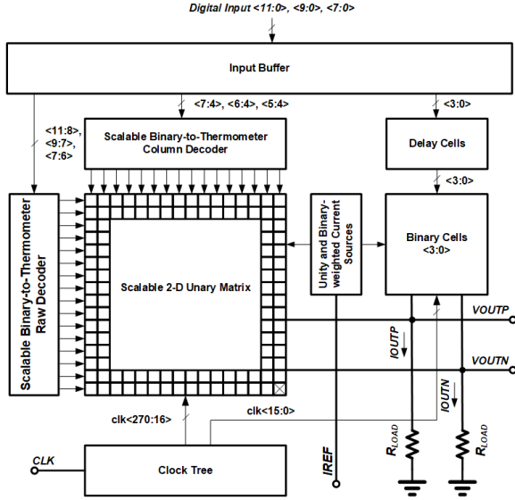
Figure 7. Proposed resolution programmable CS-DAC
