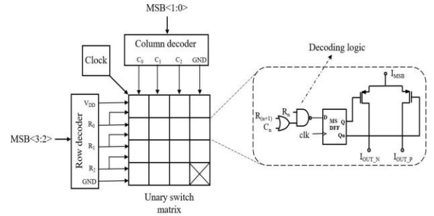
Figure 1. Example of 2D matrix architecture for 8bit resolution mode
