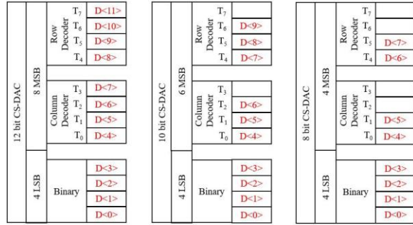
Figure 4. Proposed assignment of input digital codes
