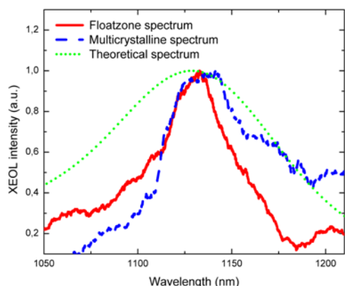
Figure 6 XEOL spectrum of floatzone silicon, spectrum of a mc silicon sample and theoretically calculated curve. The peak positions of both spectra agree well with the theoretical curve, but the width is smaller than in theory. In addition some secondary maxima are visible. The background seems to increase for longer wavelengths for the mc silicon.
