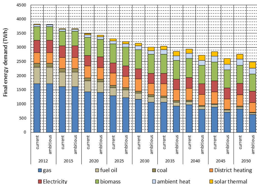
Figure 3: Shares of fossil fuels, renewables, electricity and district heating in final energy demand for space heating, hot water and space cooling supply in EU28 until 2050
