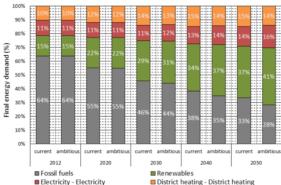
Figure 3: Shares of fossil fuels, renewables, electricity and district heating in final energy demand for space heating, hot water and space cooling supply in EU28 until 2050
