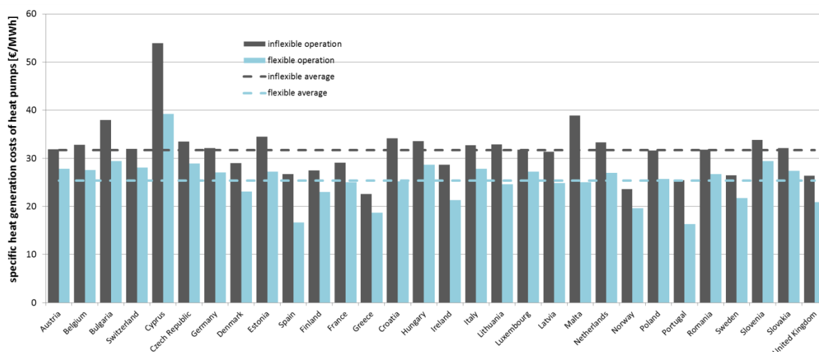
Figure 10: Specific heat generation costs 2 of heat pumps in 2050 in the ambitious policy scenario – comparison of flexible and inflexible operation of heat pumps in the Enertile® model.
