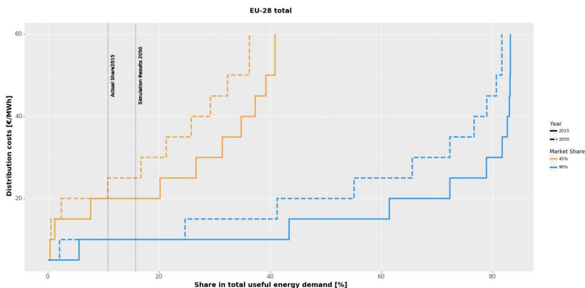
Figure 7: Estimated heat distribution costs for EU 28 in the current policy scenario for heat densities in the year 2015 and 2050 and district heating market shares of 45% and 90%
