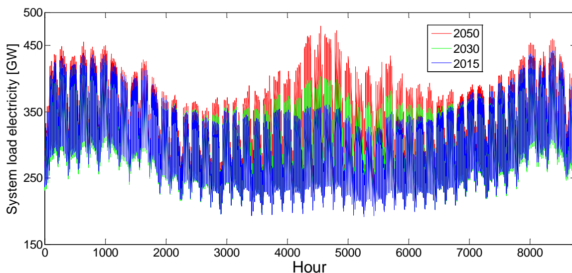
Figure 8: Change of hourly electrical load based on changes in heating and cooling demand from the current policy scenario
