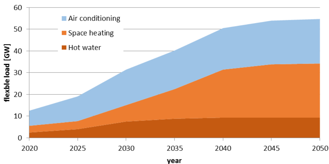
Figure 9: Uptake of flexible loads in buildings in the model EMPIRE based on heating and cooling loads from the current policy scenario
