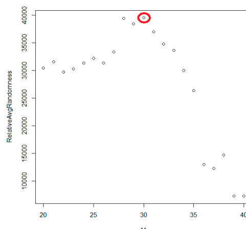
Figure 2. Considering the structure of an IP address, we defined an index of sparsity based on a random sample of IP addresses. This absolute index was relativized using a cost function exponential in the sample size. Repeated experiments showed that 30 is a good number for the size of a sample.
