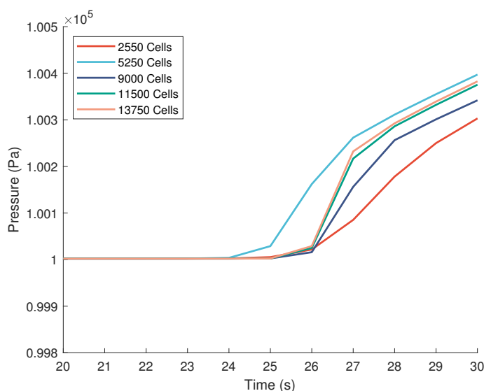
Figure A1. Convergence analysis for different amounts of cells.
