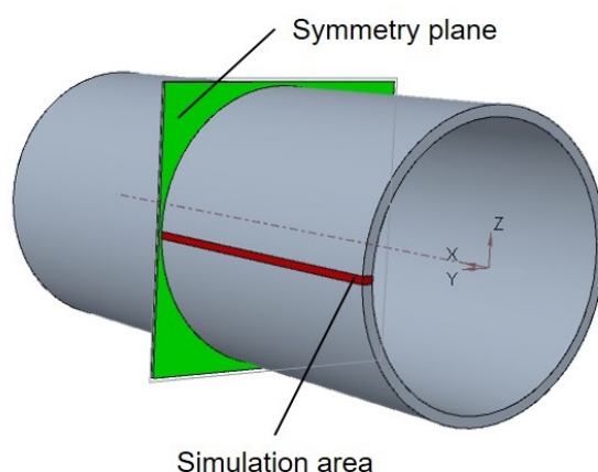
Figure 3. Simplified simulation with symmetry plane and rotation axis.
