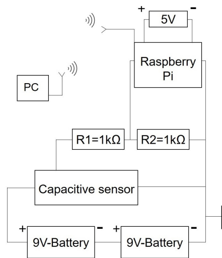
Figure 11. Electrical circuit diagram with capacitive sensor.
