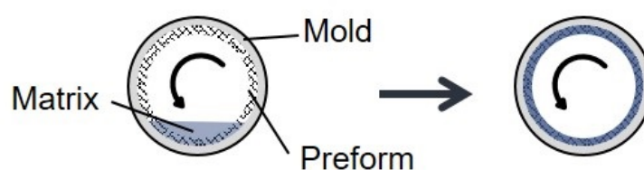
Figure 1. Simplified representation of the rotational molding process with thermoset matrix.
