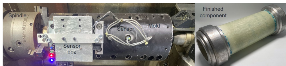
Figure 10. Mold for the rotational molding process and finished component.
