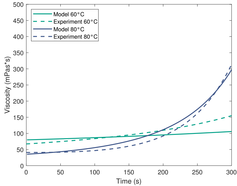
Figure 7. Comparison between viscosity \eta as a function of time of the Castro-Macosko model and the experimental measurements.
