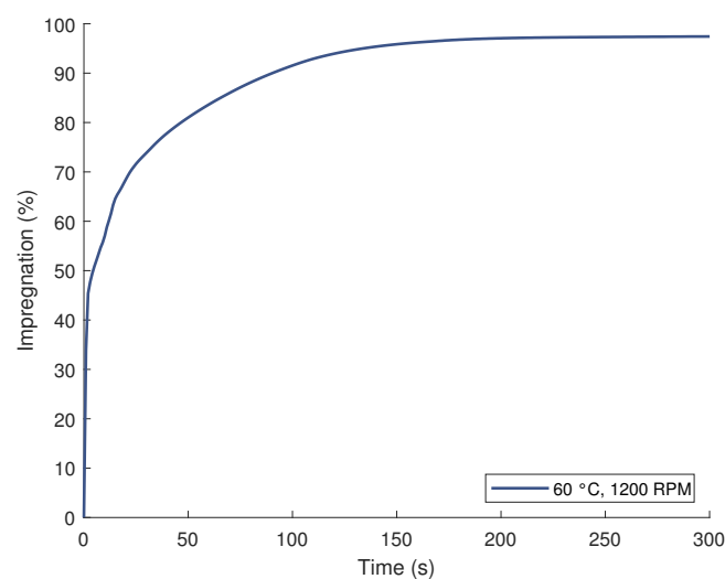
Figure 14. Impregnation progress over time.
