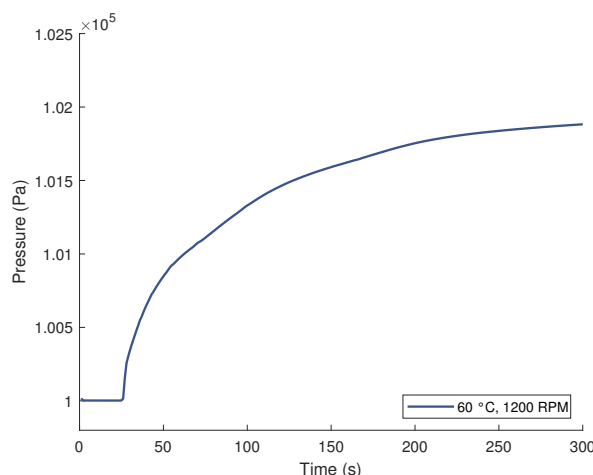
Figure 15. Simulated pressure curve at the position of the sensor after starting the rotation.
