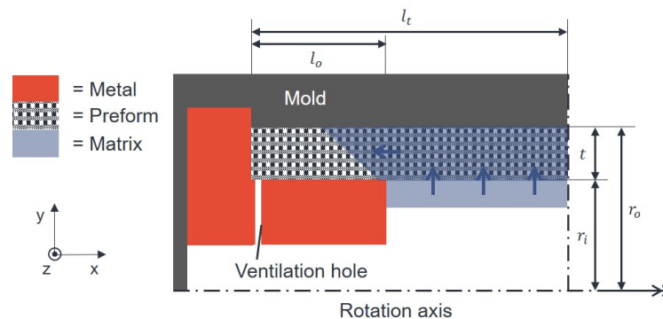
Figure 2. Impregnation in the rotational molding process [10].
