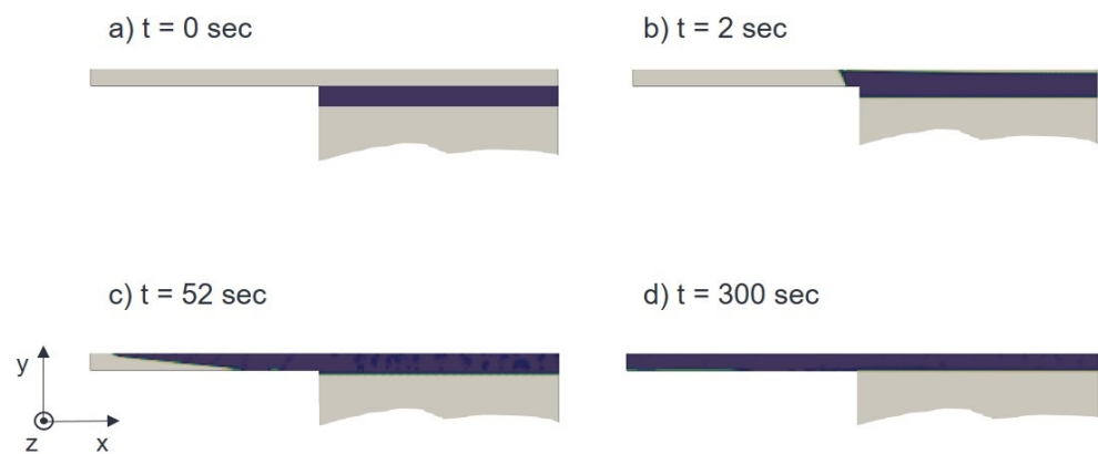
Figure 13. Different stages of impregnation for 60 °C and 1200 RPM.
