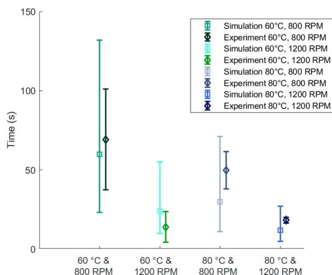
Figure 16. Comparison of the experimentally measured times with the numerically calculated times for reaching the sensor with the matrix.
