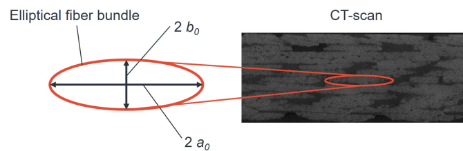
Figure 8. Determination of the equivalent radius of the fiber bundles r_{eq} by computed tomography studies of the cross section
