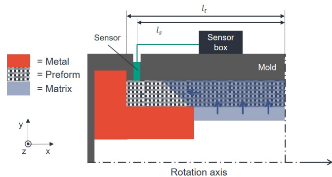
Figure 12. Sensor integration into the mold.
