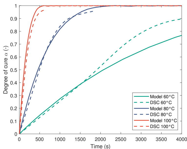
Figure 6. Degree of cure \alpha as a function of time fitted to isothermal DSC data.
