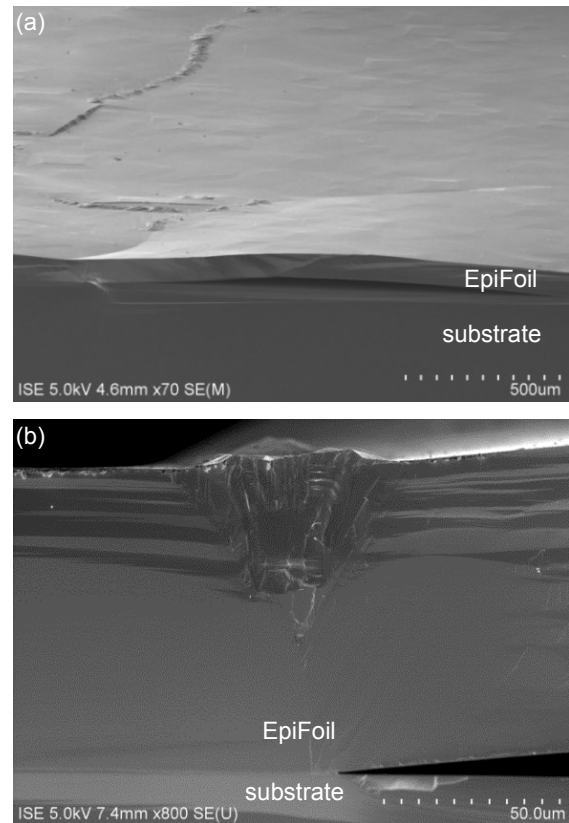
Figure 5: Local warping of the reorganized template leading to (a) sticking of the silicon EpiFoil at the edges of the warped area, and (b) formation of defects (stacking faults).
