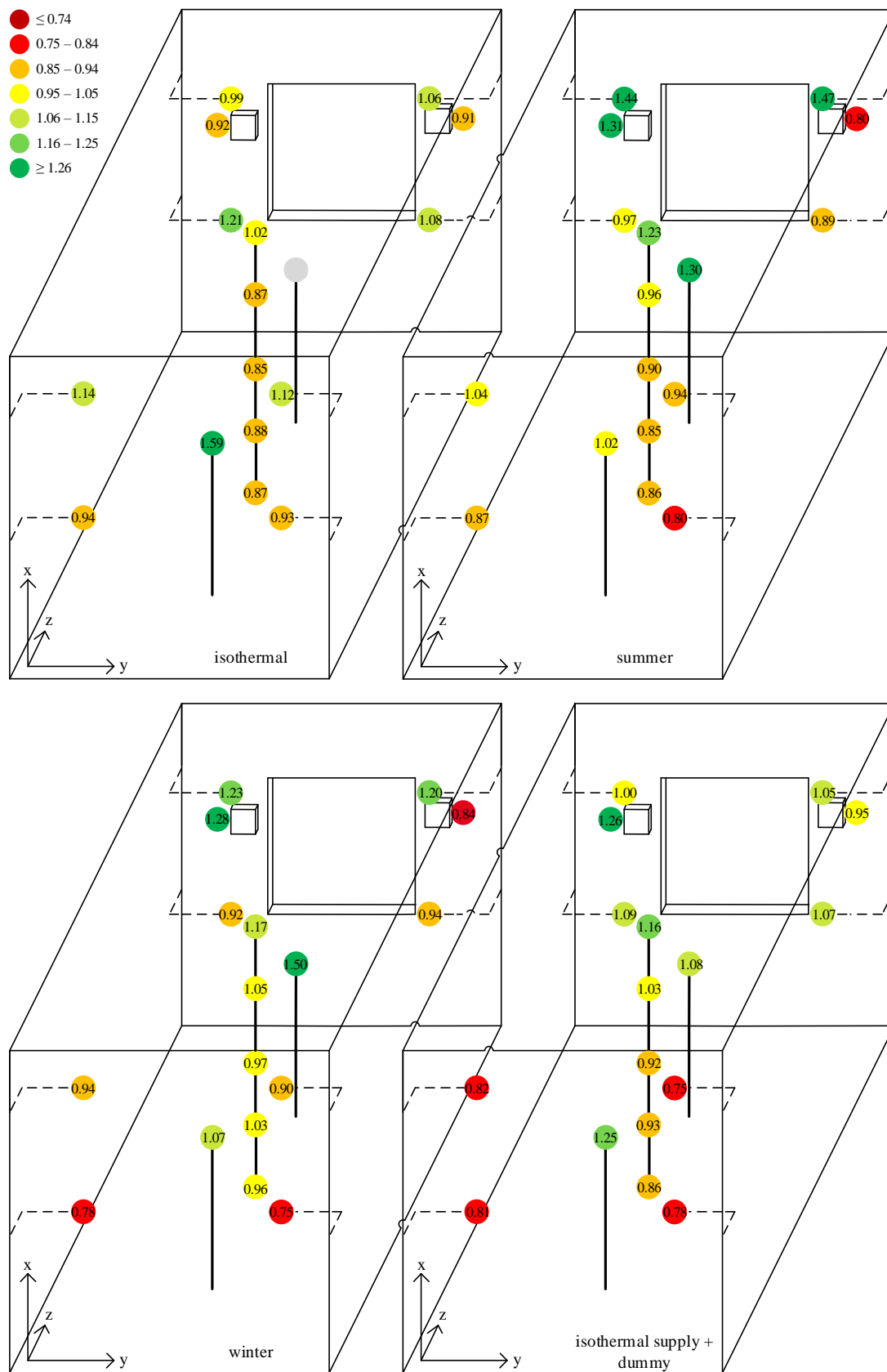
Figure 7. Local air exchange indices \epsilon^a_{Nj} (2–3) at \dot{V} = 28 \text{ m}^3 \cdot \text{h}^{-1} : isothermal (top left), summer (top right), winter supply air conditions (bottom left), isothermal supply air conditions plus placement of a dummy to simulate human heat dissipation of 300 W (bottom right) [36].
